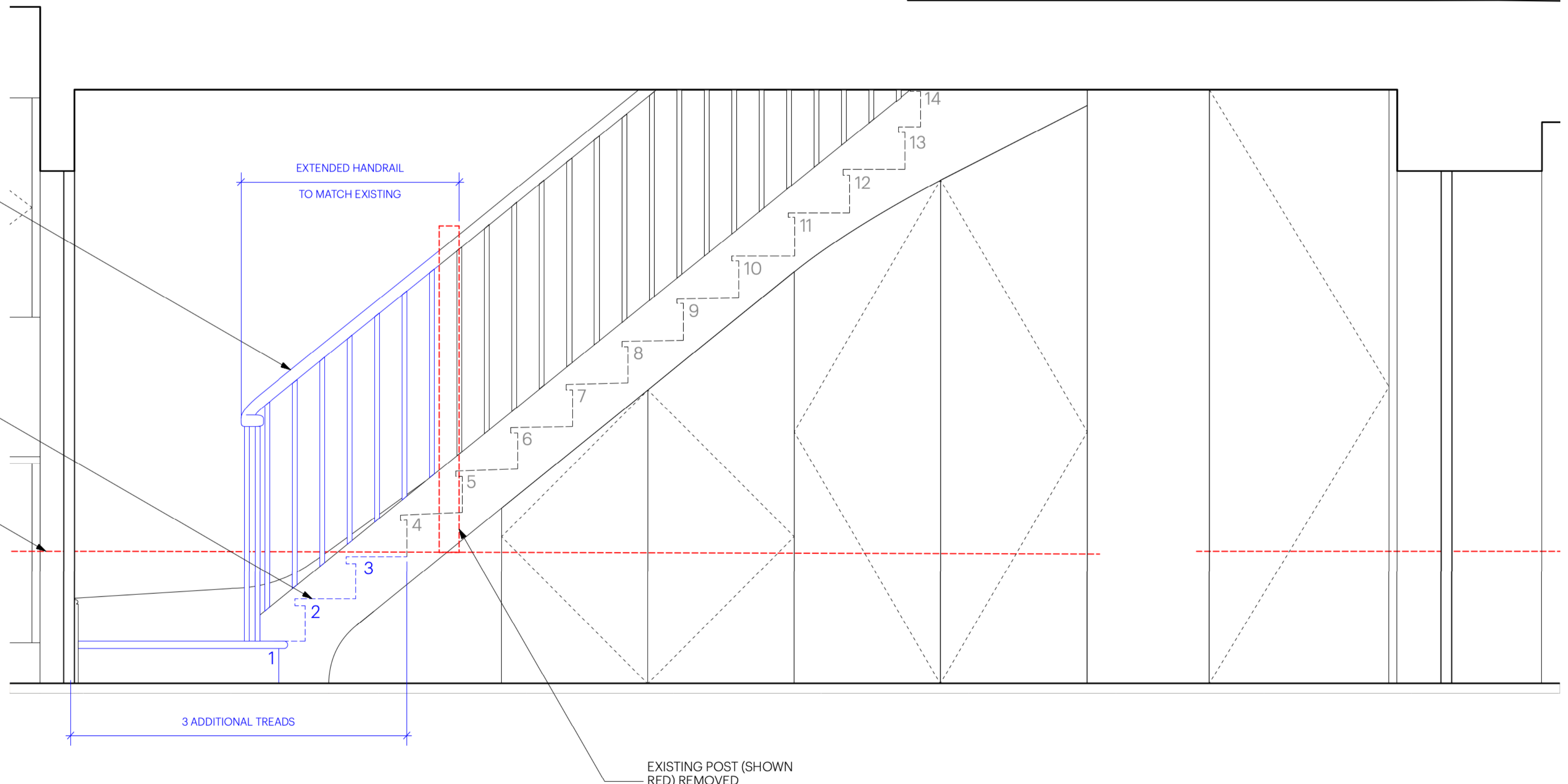
2 PROPOSED SECTION BB Scale: 1:12.5
