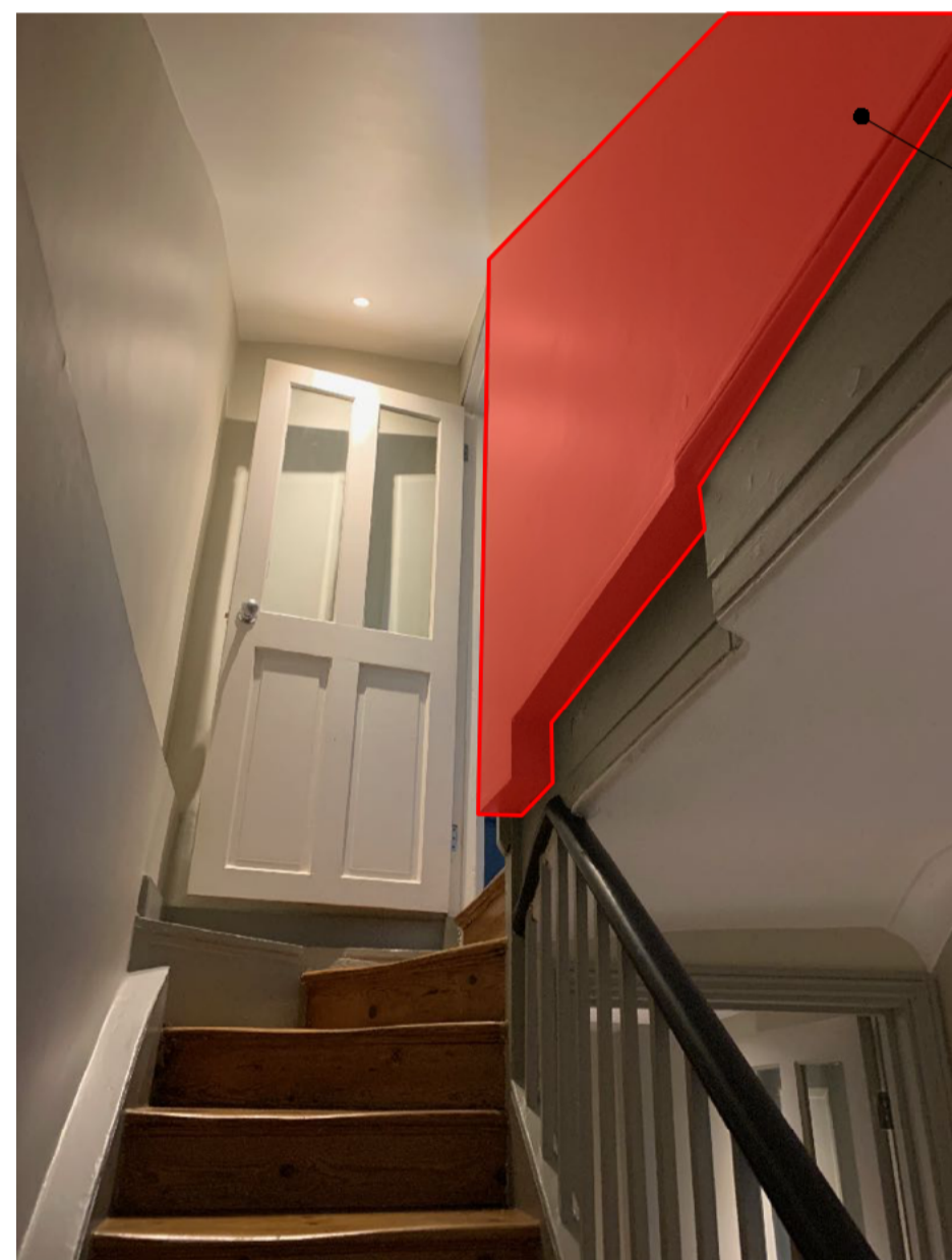
EXISTING UGF/LGF STAIRCASE
