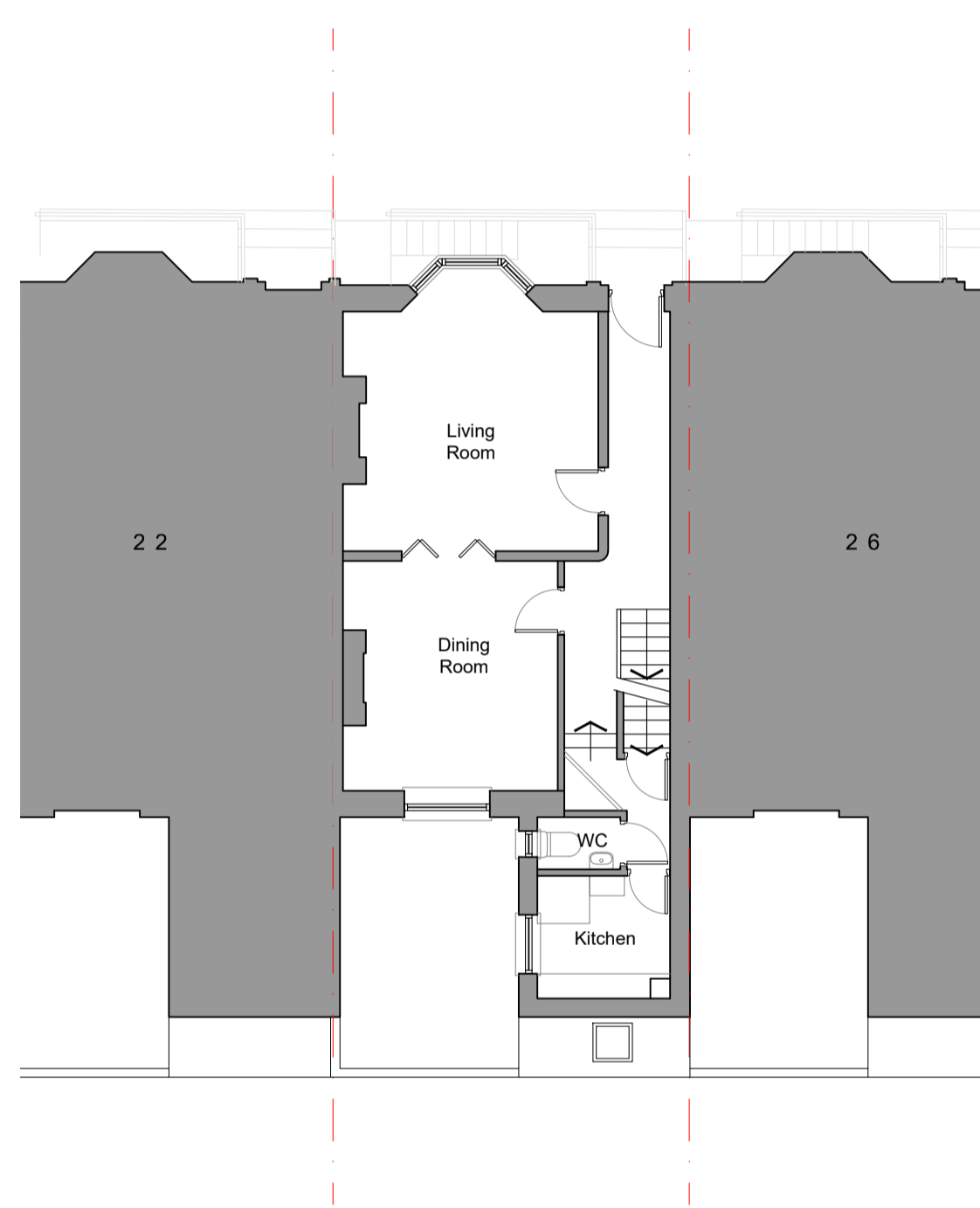
02 Ground Floor Plan Scale:1:100
