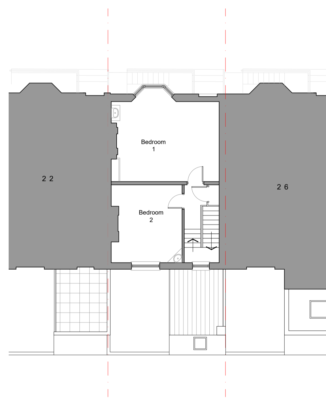
03 First Floor Plan Scale:1:100
