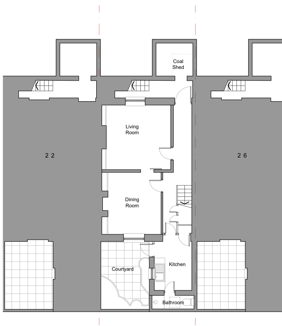
01 Lower Ground Floor Plan Scale:1:100
