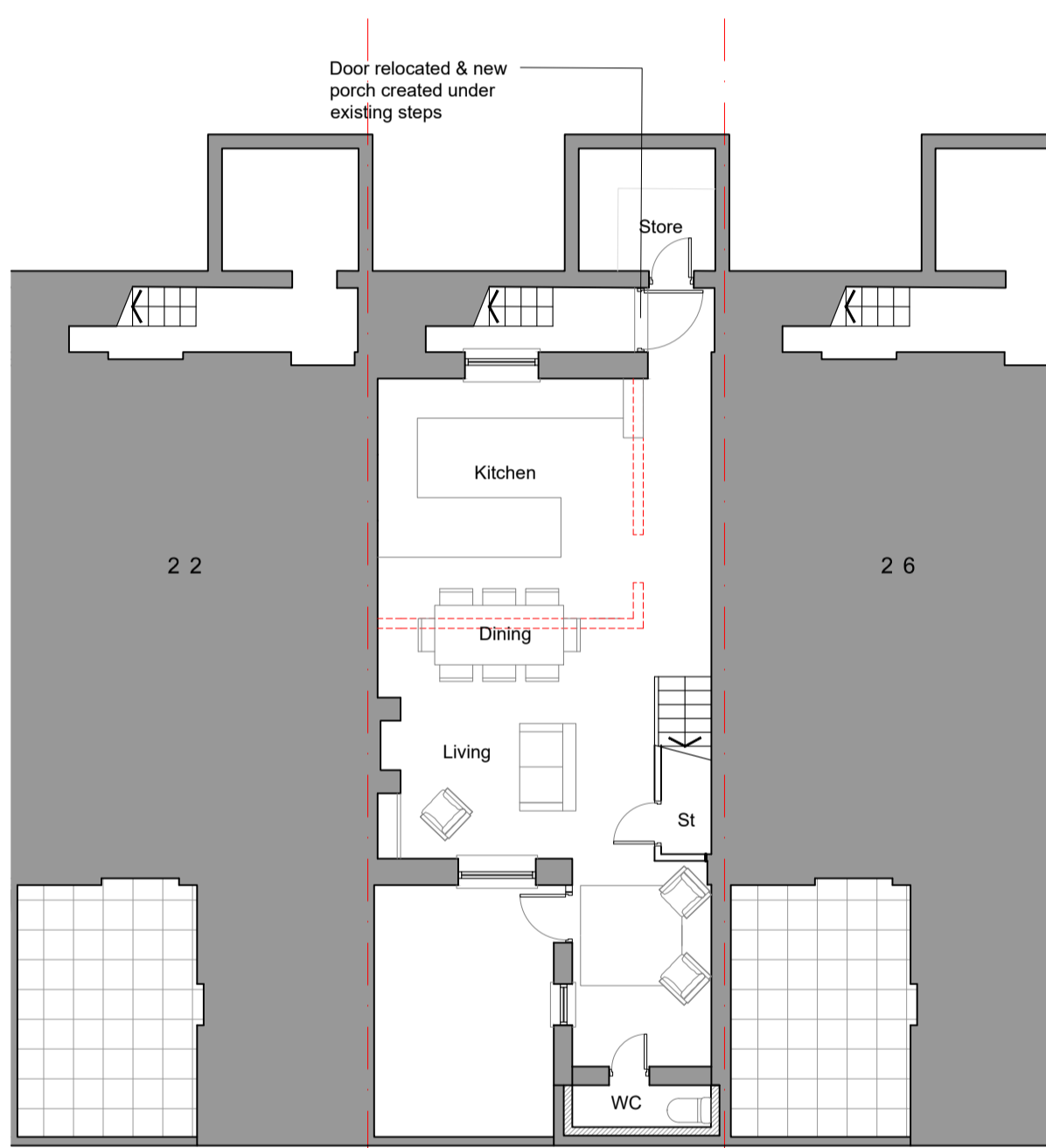
01 Lower Ground Floor Plan Scale:1:100
