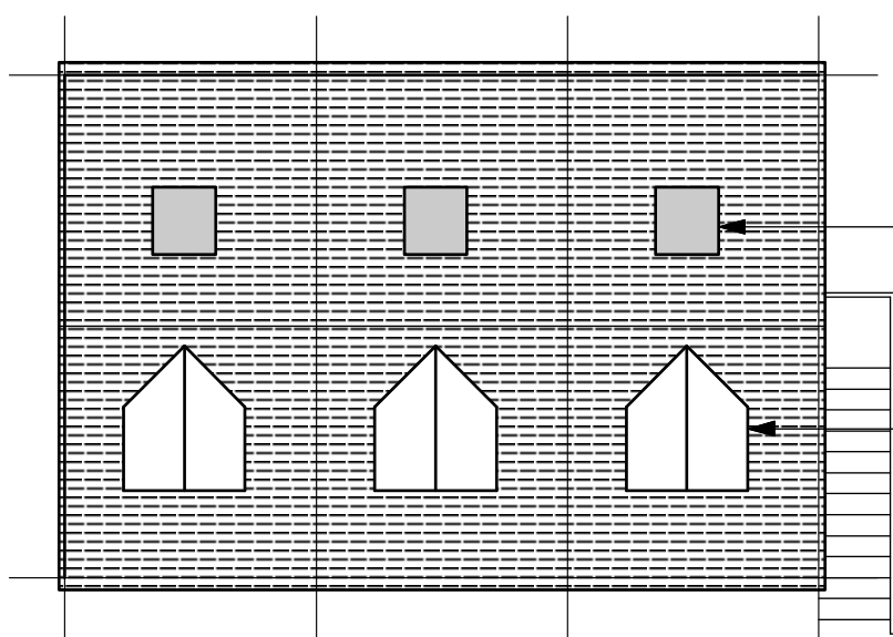
Garage Block Roof Plan
