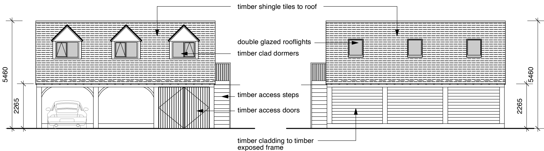
Front Elevation of Garage Block
