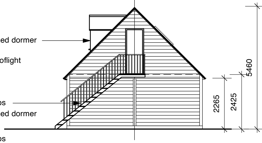
East Elevation of Garage Block
