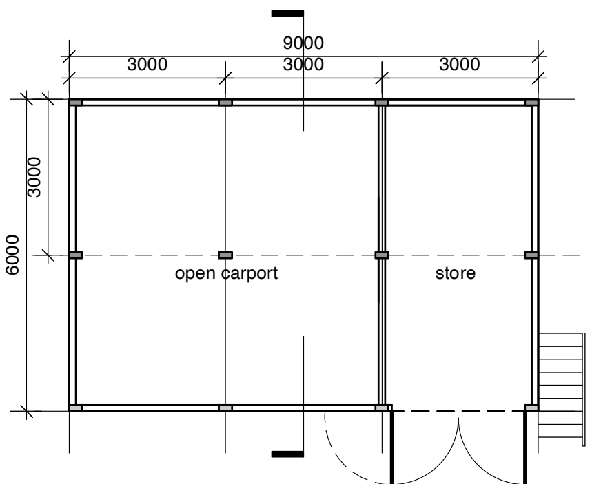
Garage Block Layout Plan
