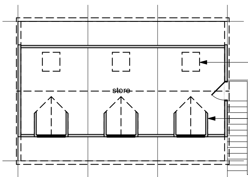
Upper Storage Layout Plan
