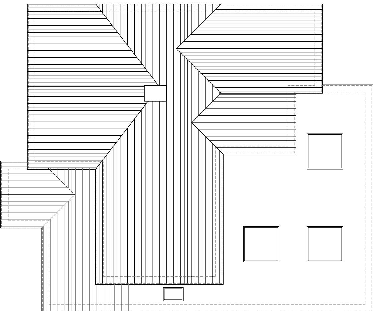
Roof Plan As Proposed
