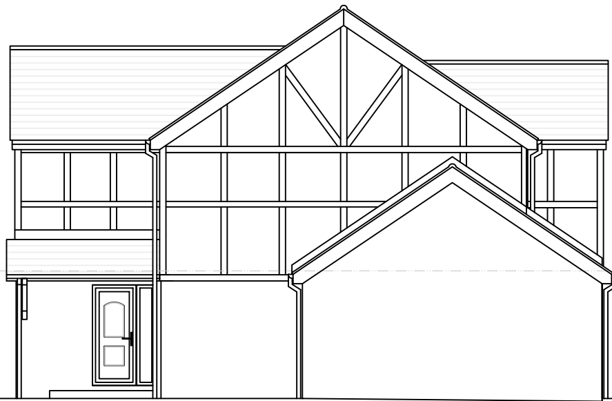
EXISTING ELEVATION B - SIDE
