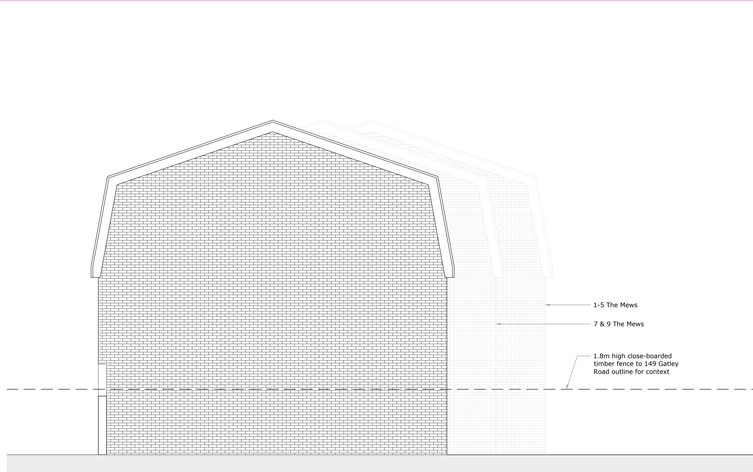
side elevation (east facing) as existing 1:50
