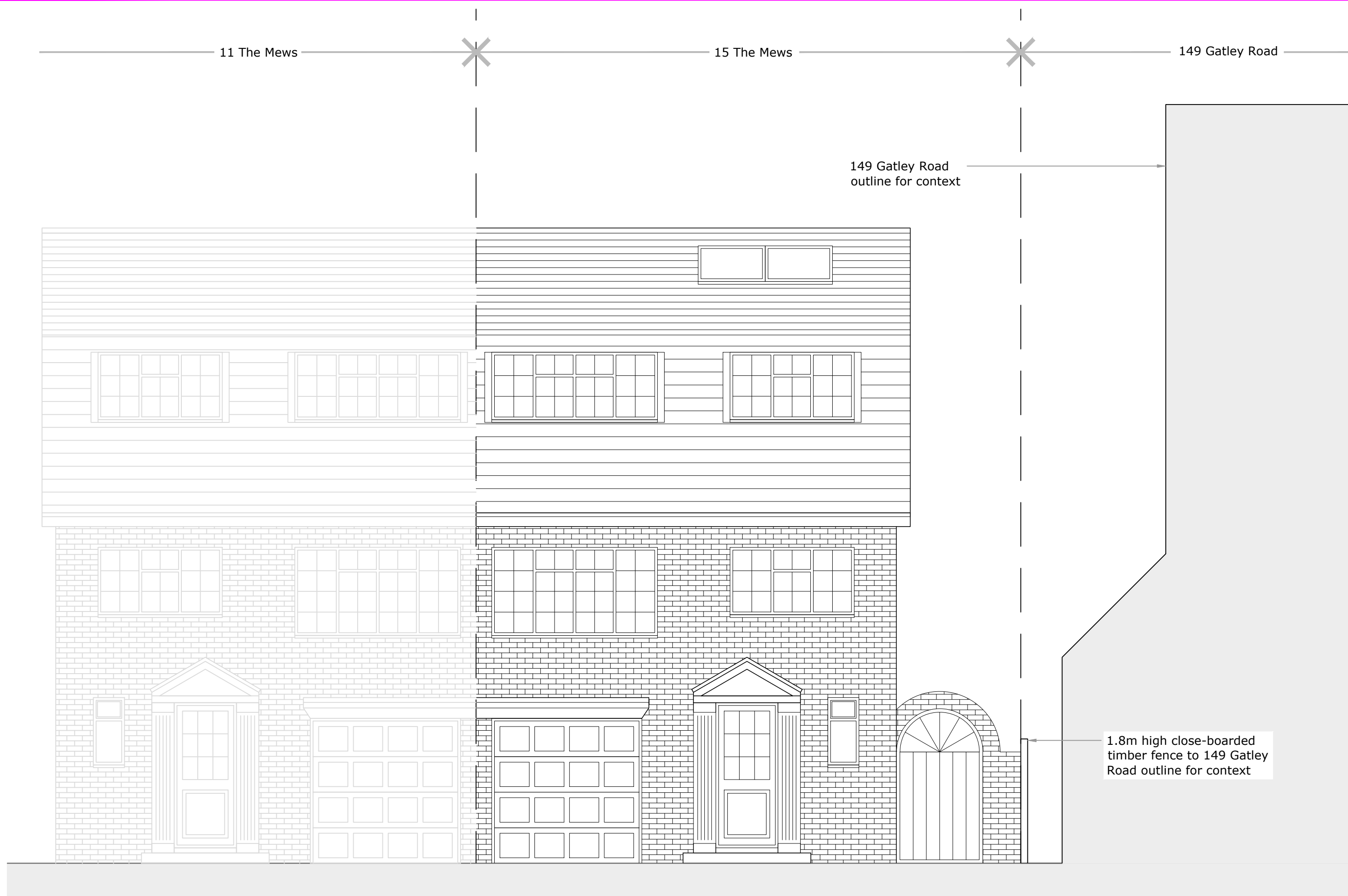
front elevation (south facing) as existing 1:50
