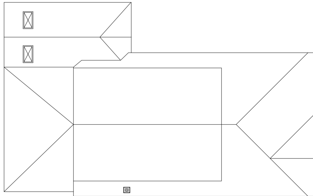
3 PROPOSED ROOF PLAN 1:100
