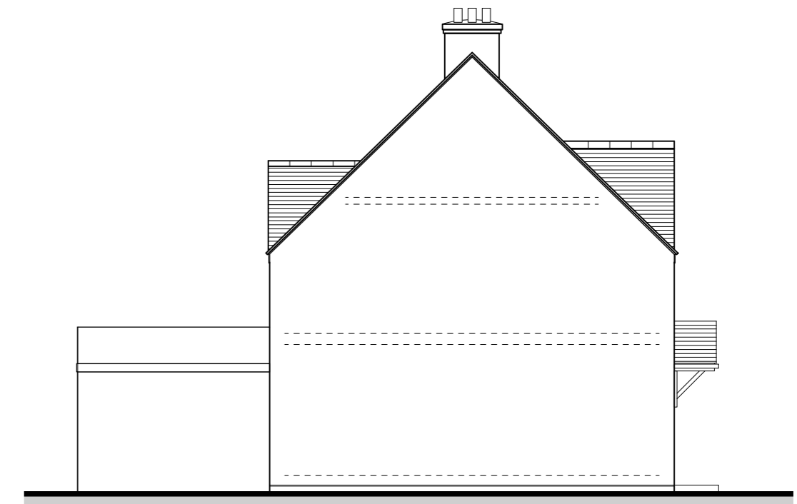
03 EXISTING SIDE ELEVATION (SECTION CUT) 06 SCALE 1:50 @A2
