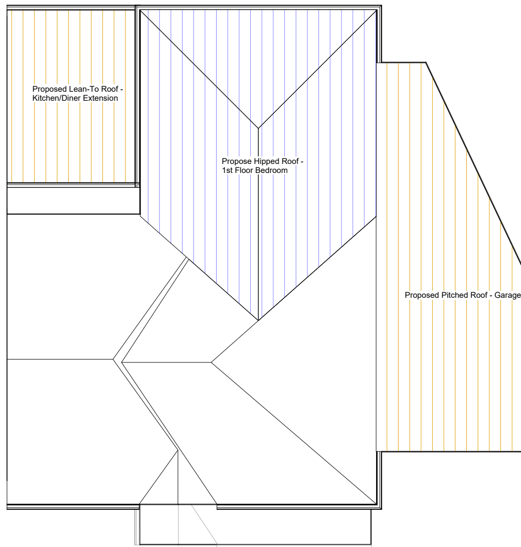
1 RF - Proposed Roof Plan SS 1 : 100
