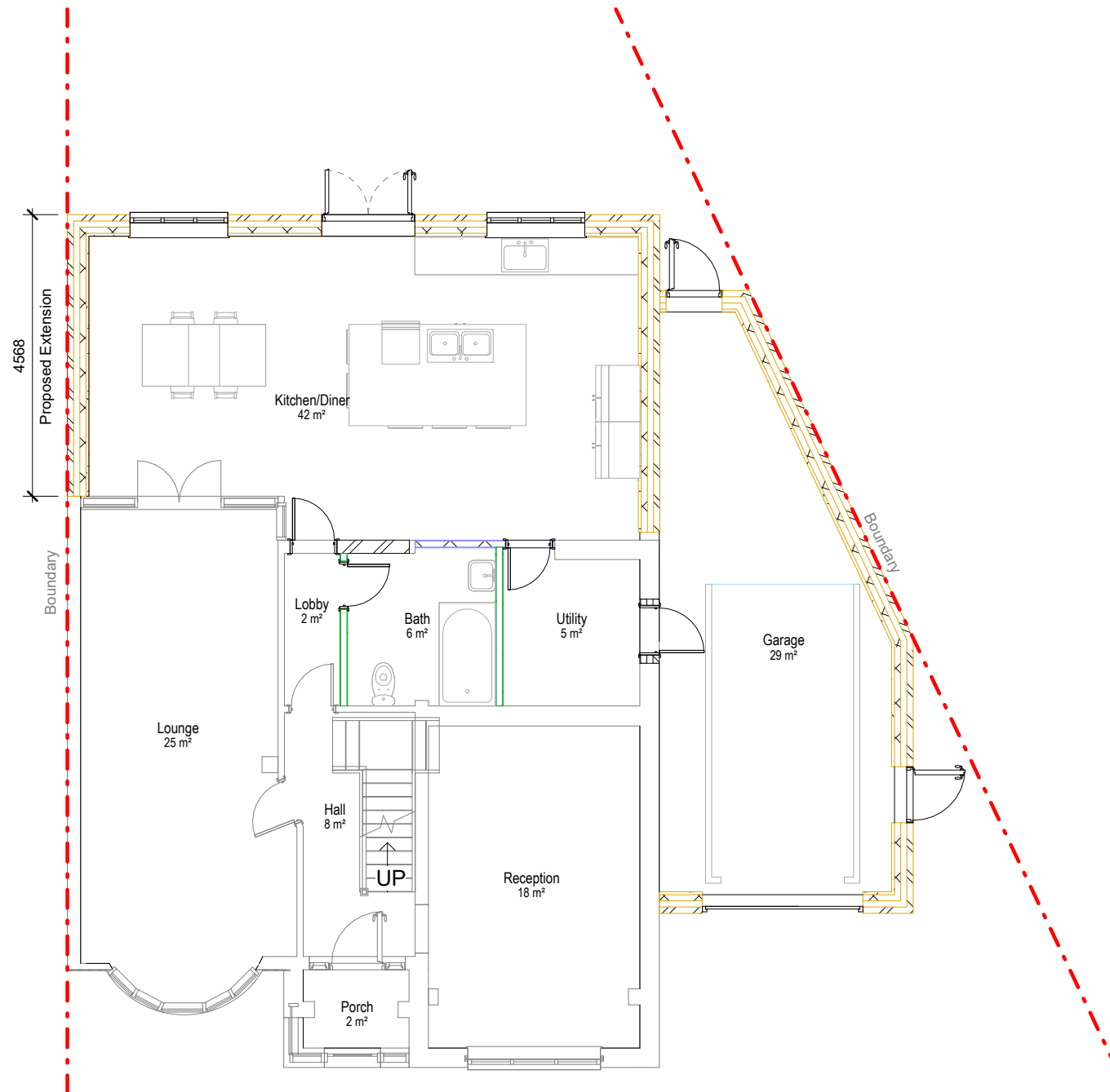
1 00 - Proposed Ground Floor Plan SS 1 : 100
