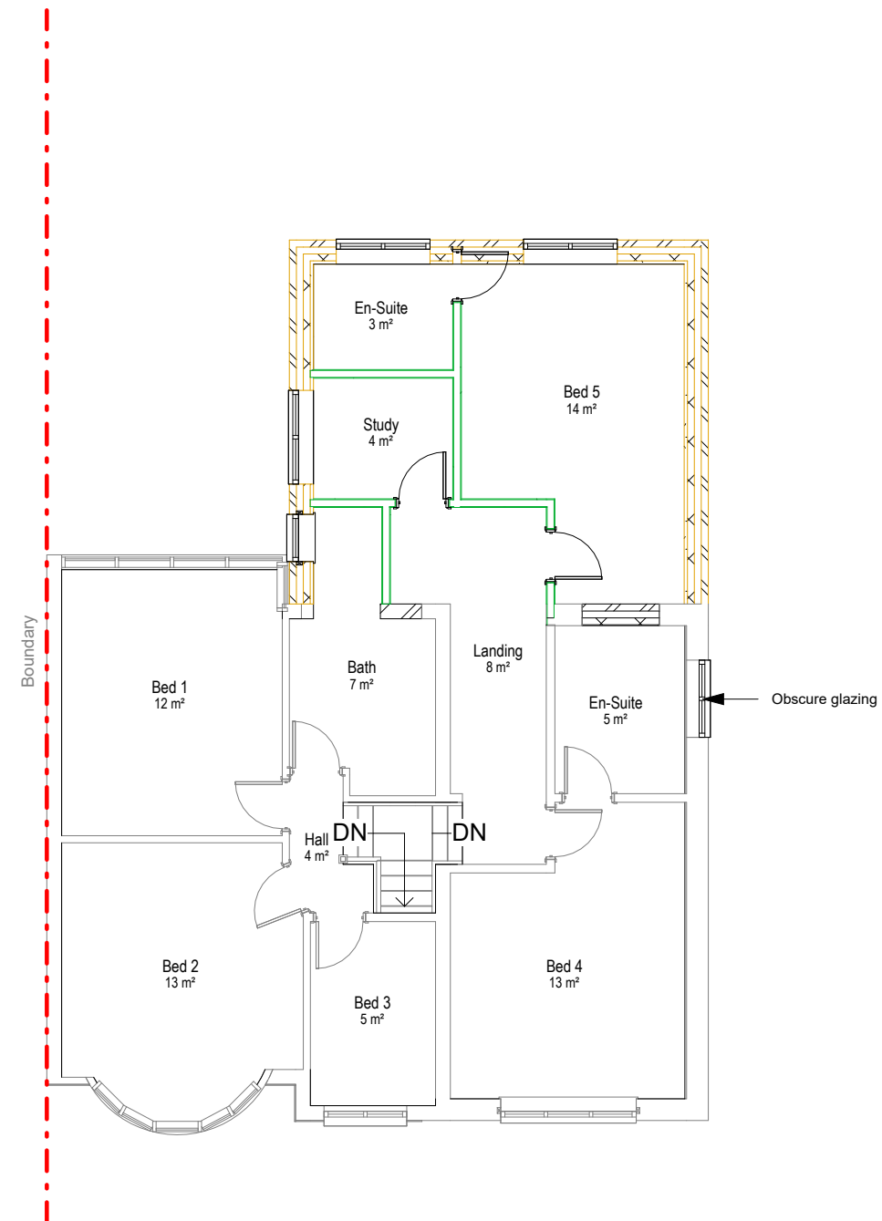
2 01 - Proposed First Floor Plan SS 1 : 100
