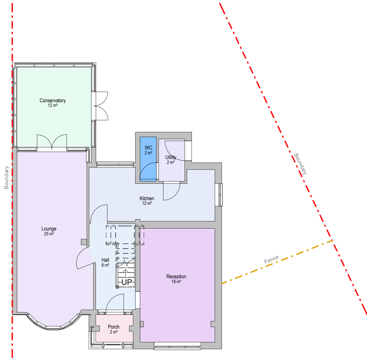
1 00 - Existing Ground Floor Plan 1 : 100
