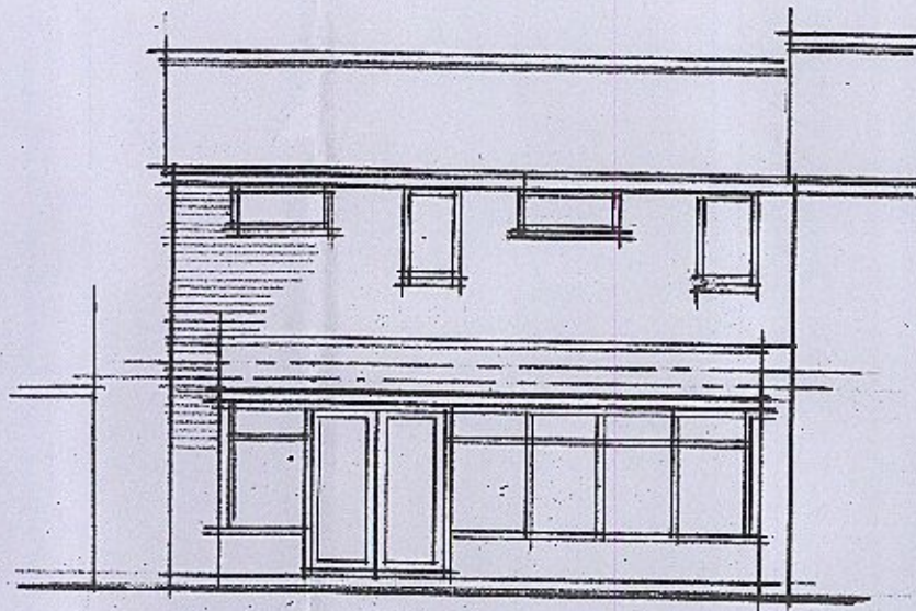
REAR ELEVATION 1:100
