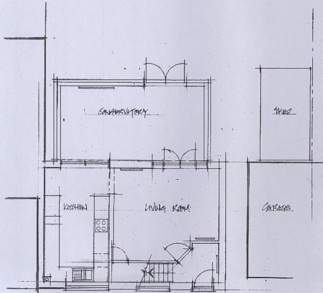
EXISTING PLAN 1:100
