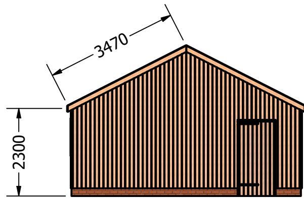
South Elevation
