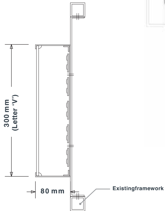
SECTIONTHROUGH- Scale 1:5
