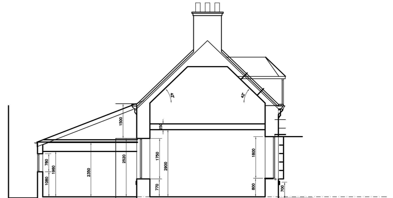
Section
