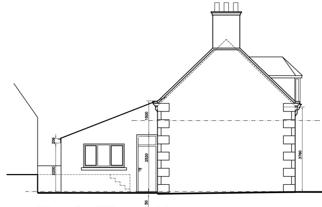
East Elevation
