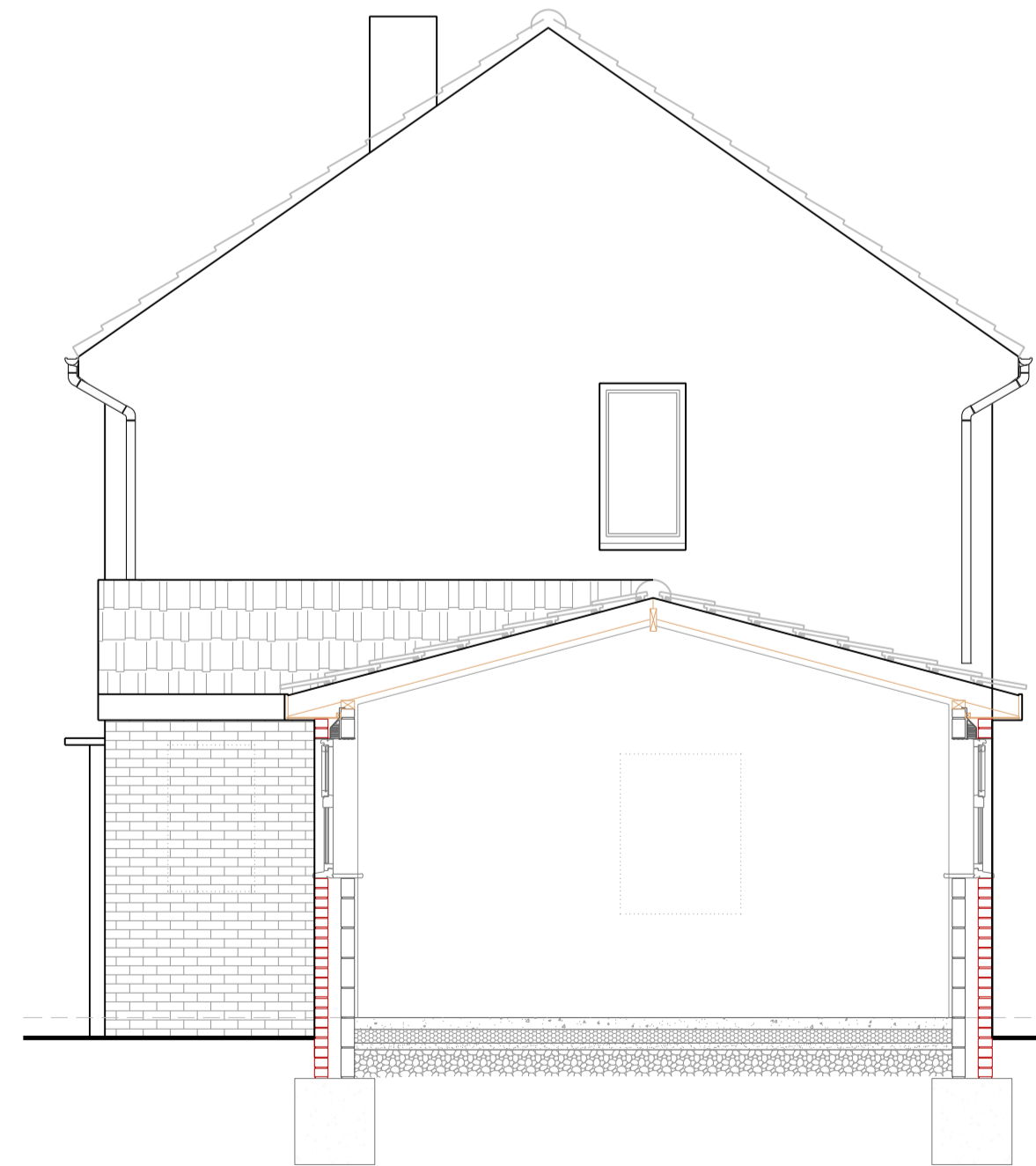
PROPOSED SECTION A:A - 1:50
