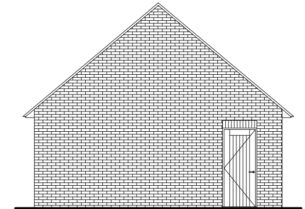
PROPOSED SIDE (SE) ELEVATION (1:100)
