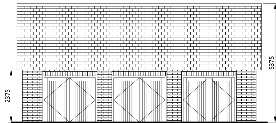
PROPOSED FRONT (NE) ELEVATION (1:100)
