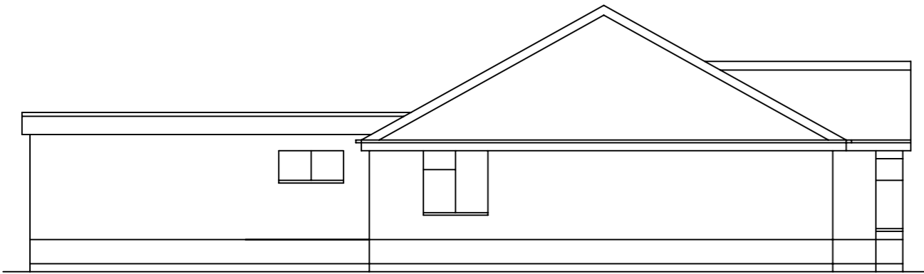
PROPOSED EAST ELEVATION ( Side )
