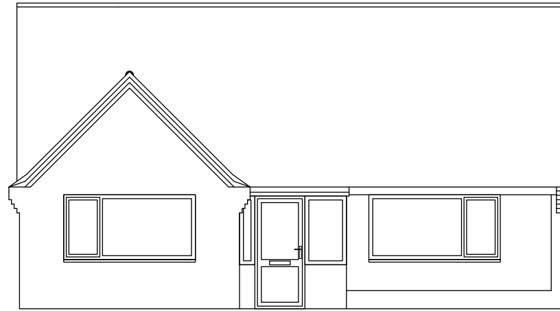
NORTH ELEVATION
