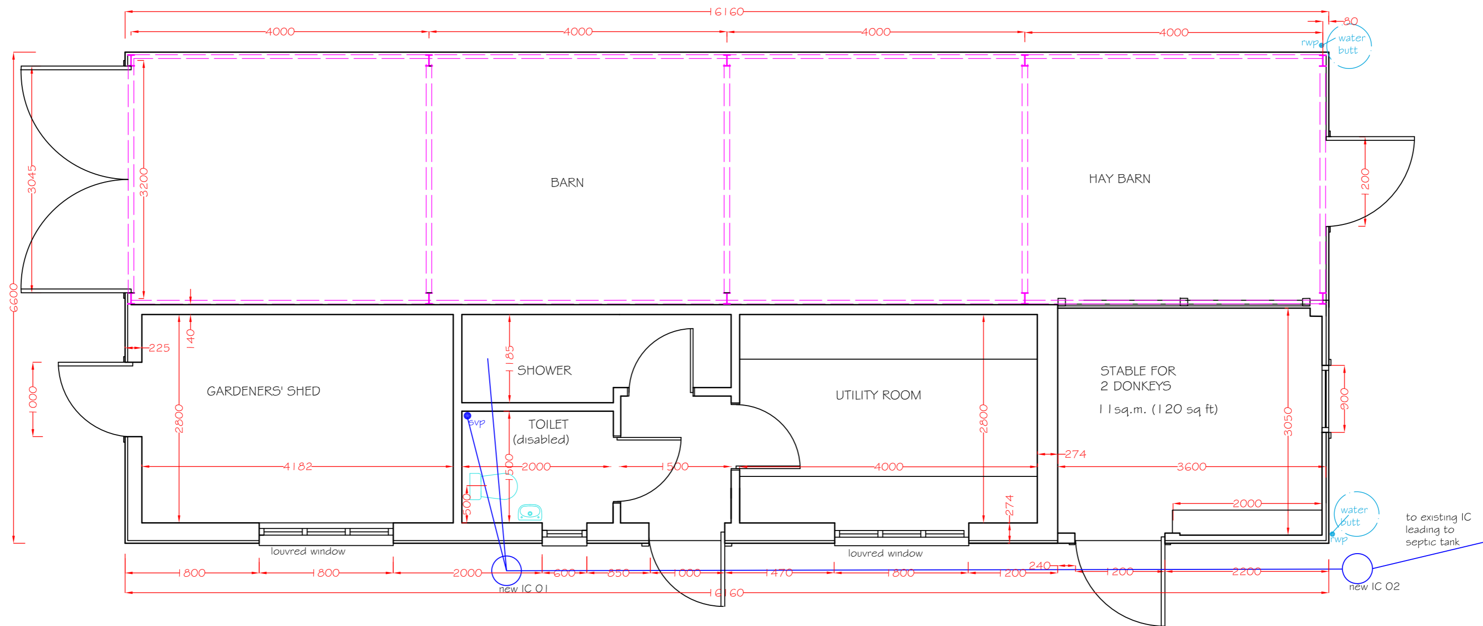
FLOOR PLAN scale 1:50
