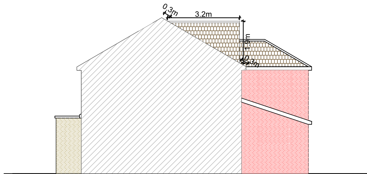
PROPOSED SIDE ELEVATION - B
