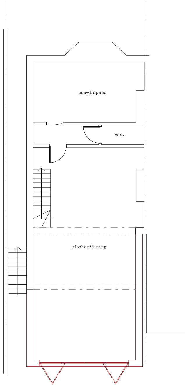
PROPOSED BASEMENT FLOOR PLAN
