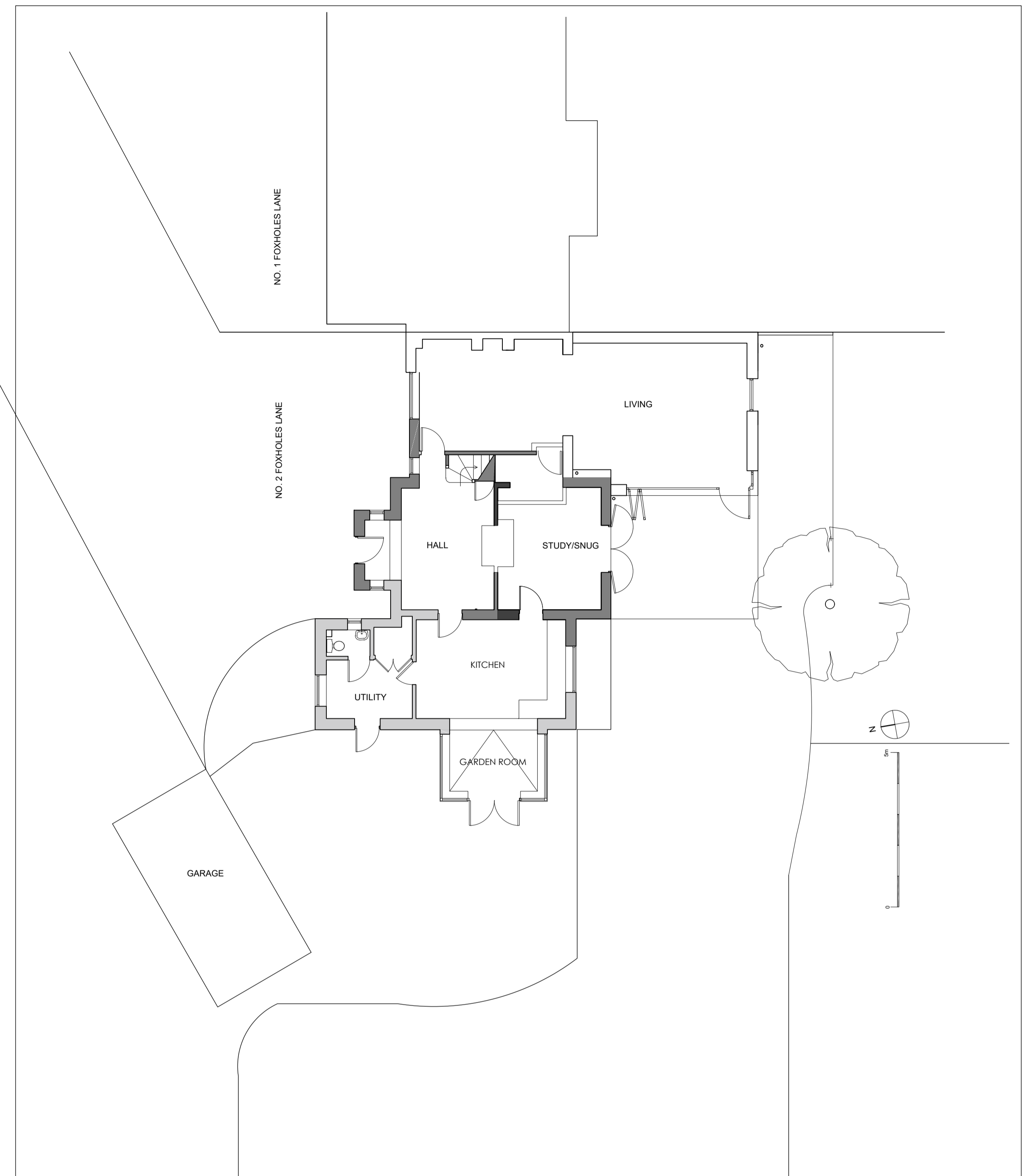
GROUND FLOOR 1:100
