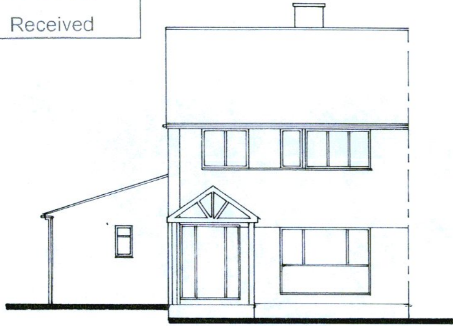
Front Elevation
