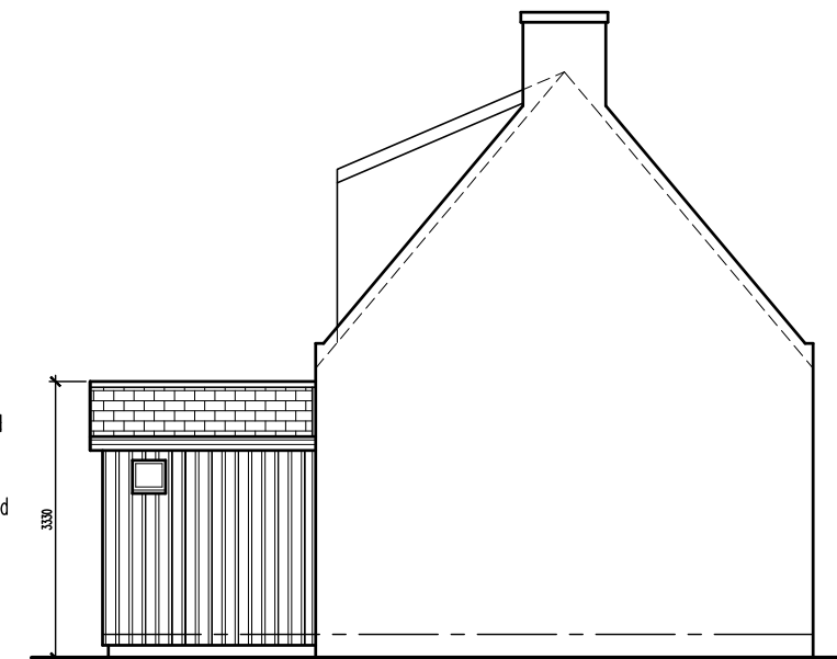
EAST ELEVATION
