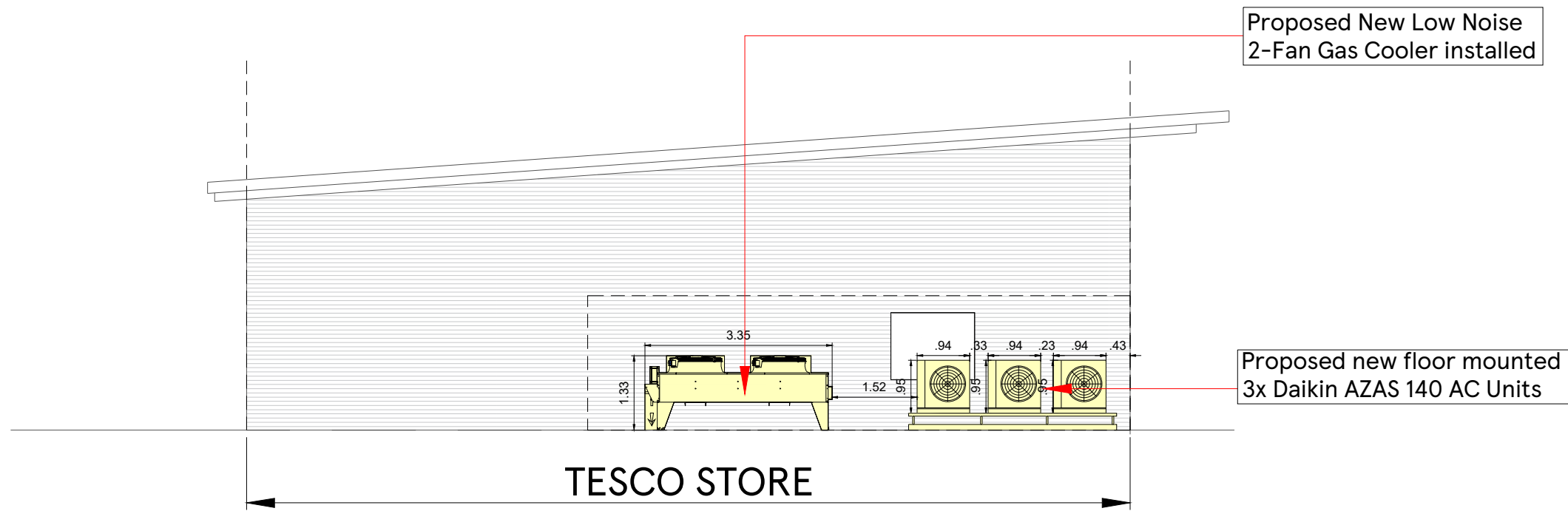
EAST ELEVATION WITH FENCE HIDDEN
