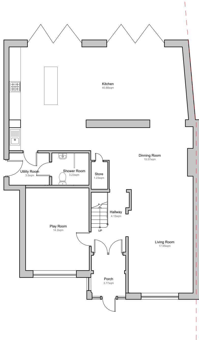
GROUND FLOOR
