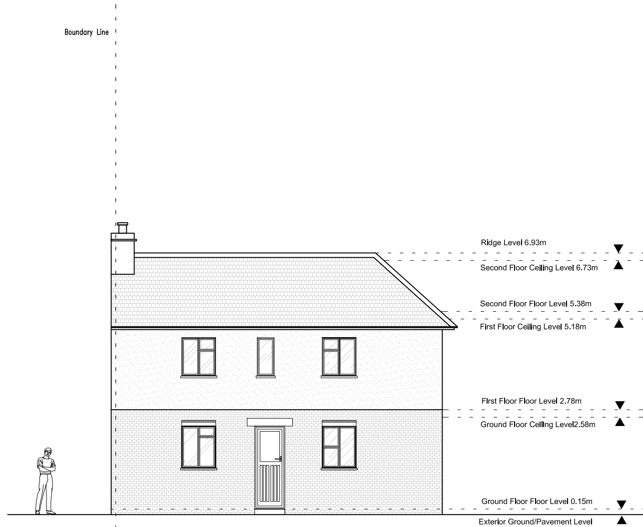
Proposed Front Elevation 1-100@A3
