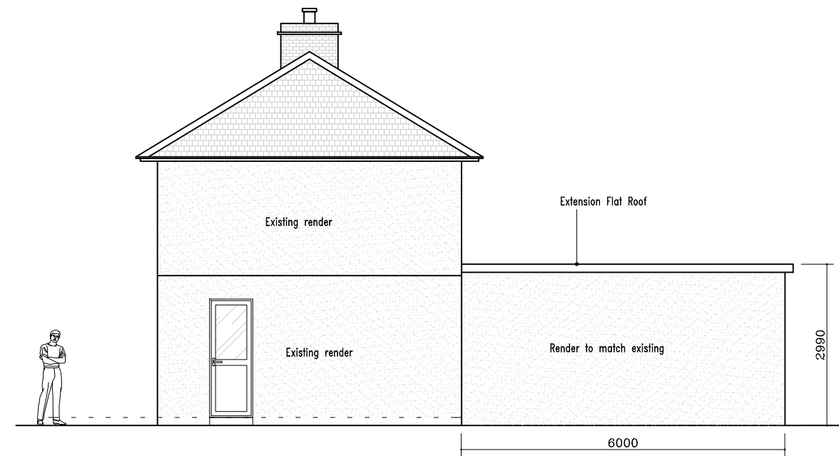
Proposed Right Elevation 1-100@A3
