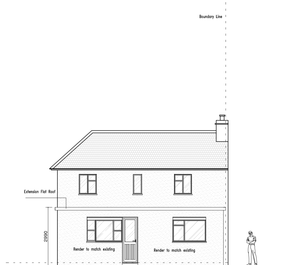
Proposed Back Elevation 1-100@A3
