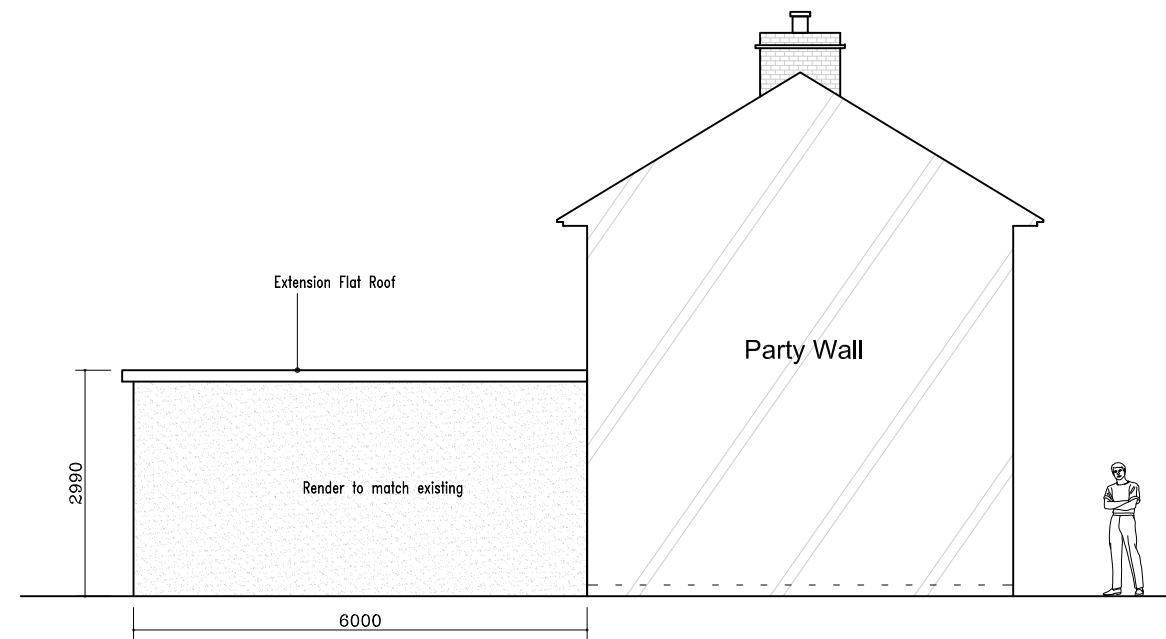
Proposed Left Elevation 1-100@A3
