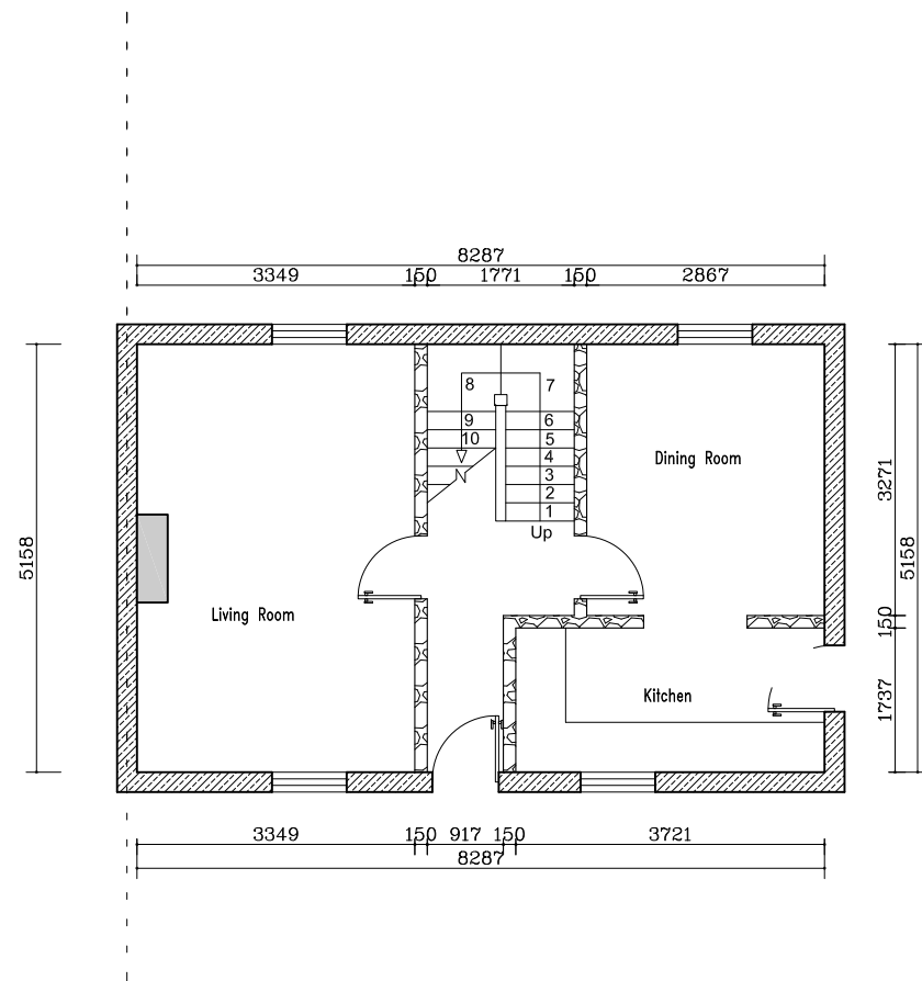
Existing Ground Floor 1-100 @ A3
