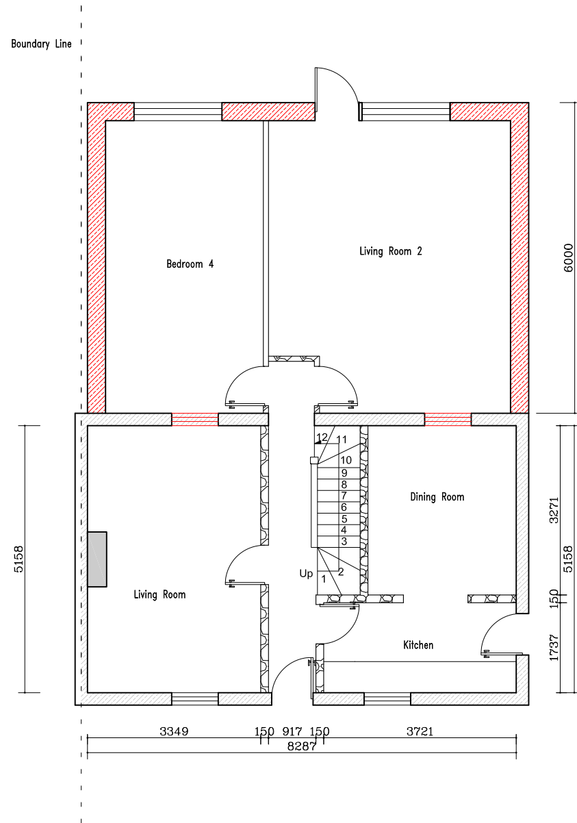
Proposed Ground Floor 1-100 @ A3
