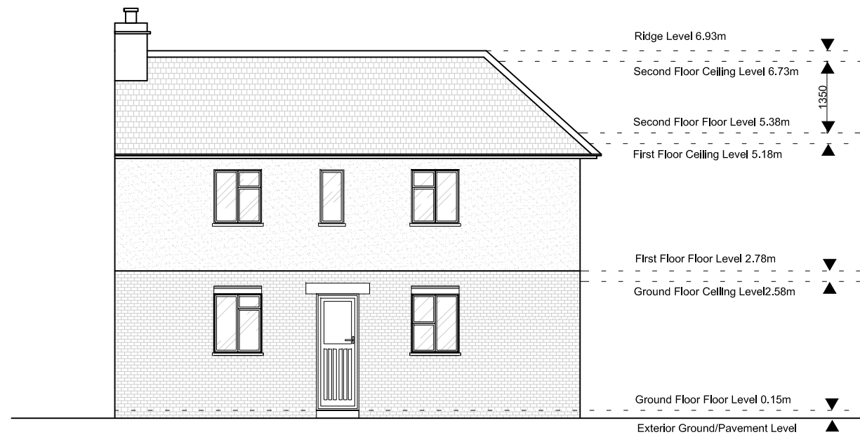
Existing Front Elevation 1-100@A3
