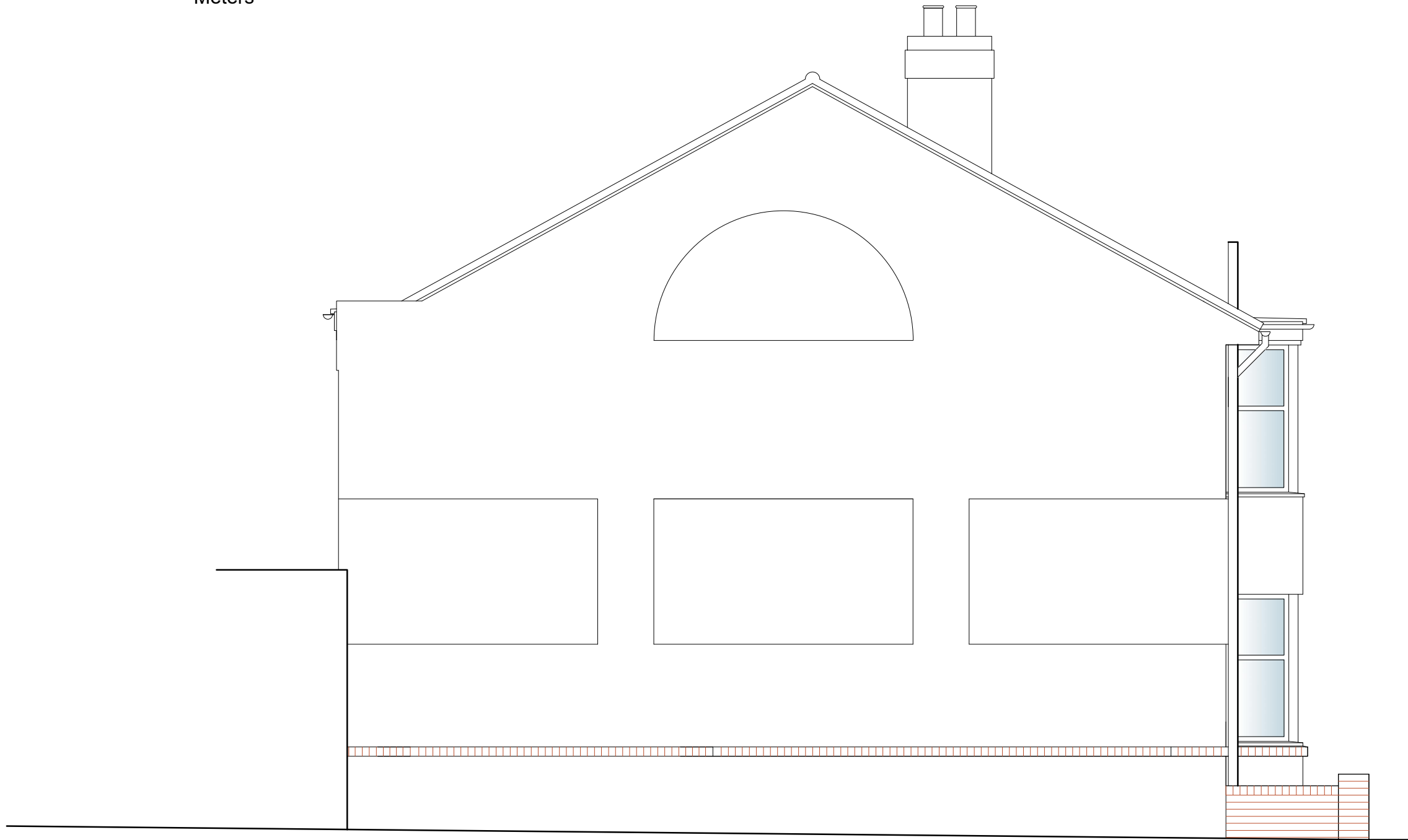
Existing Side Elevation -East
