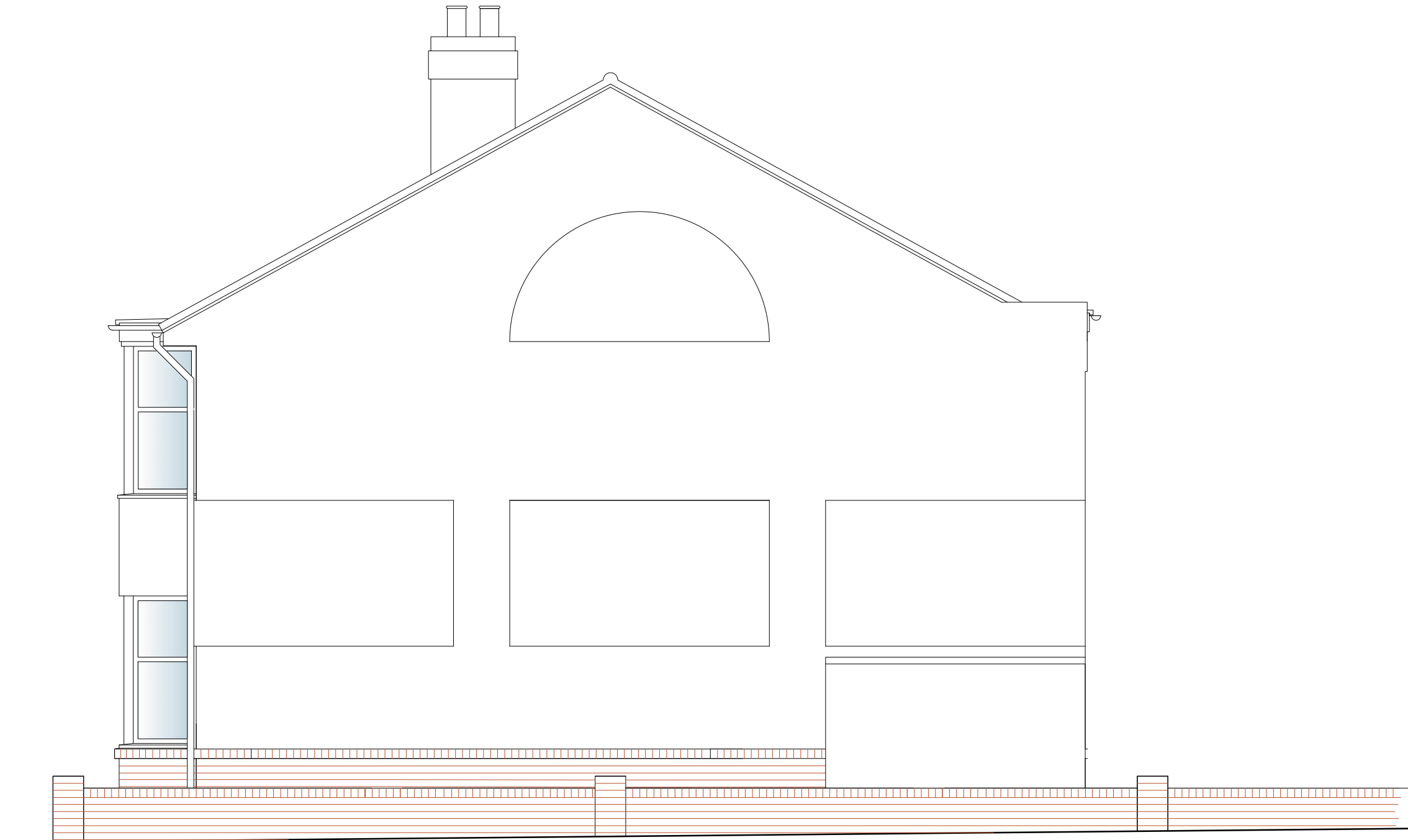
Existing Side Elevation - West
