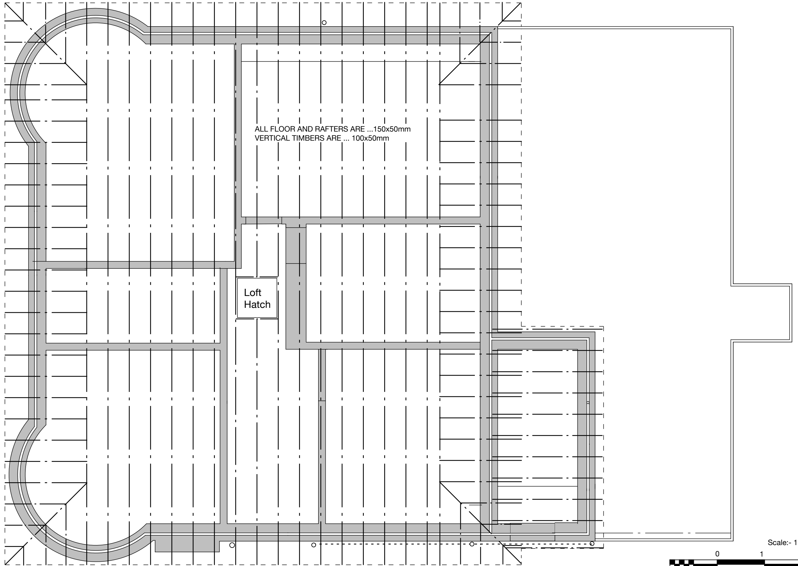
CEILING JOIST PLAN...
