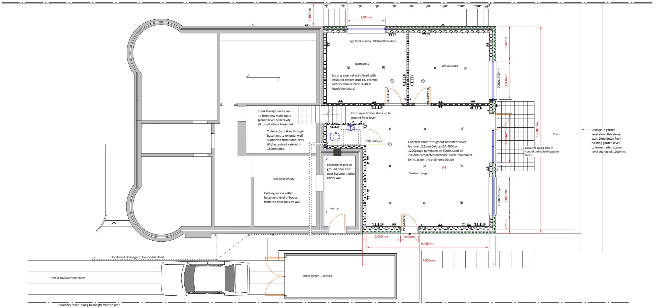
BASEMENT PLAN... 81.82 Sq m
