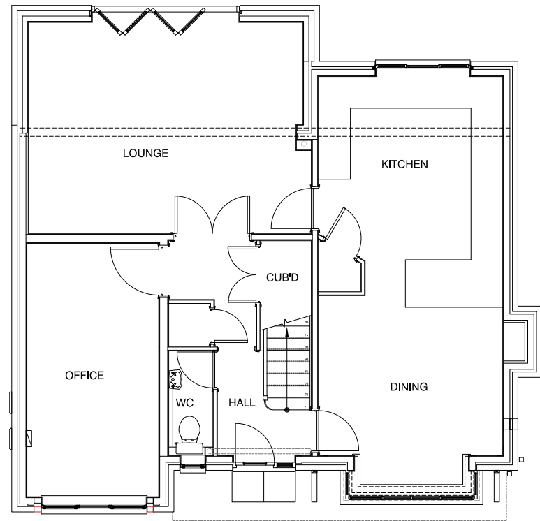
GF PLAN
