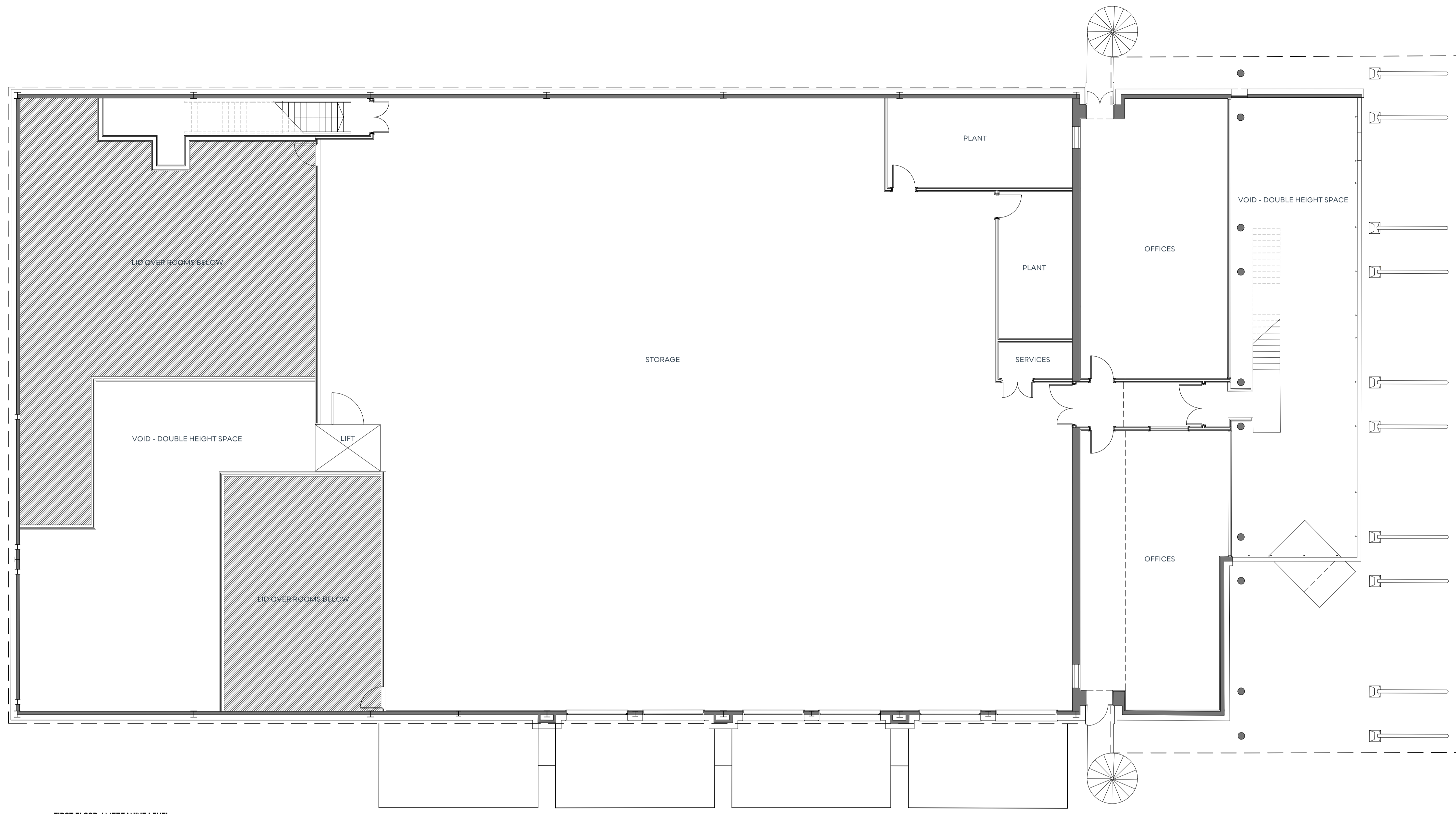
◆ FIRST FLOOR / MEZZANINE LEVEL @ 1:100
