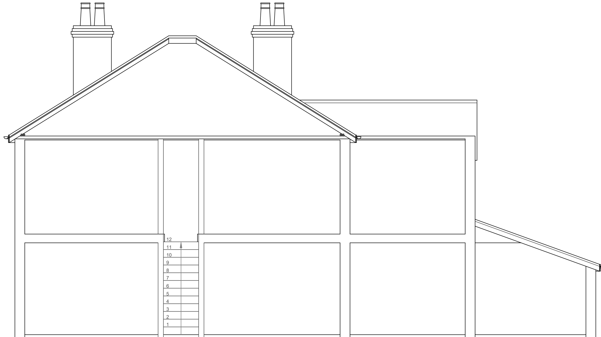
EXISTING CROSS SECTION: AA SCALE 1:50
