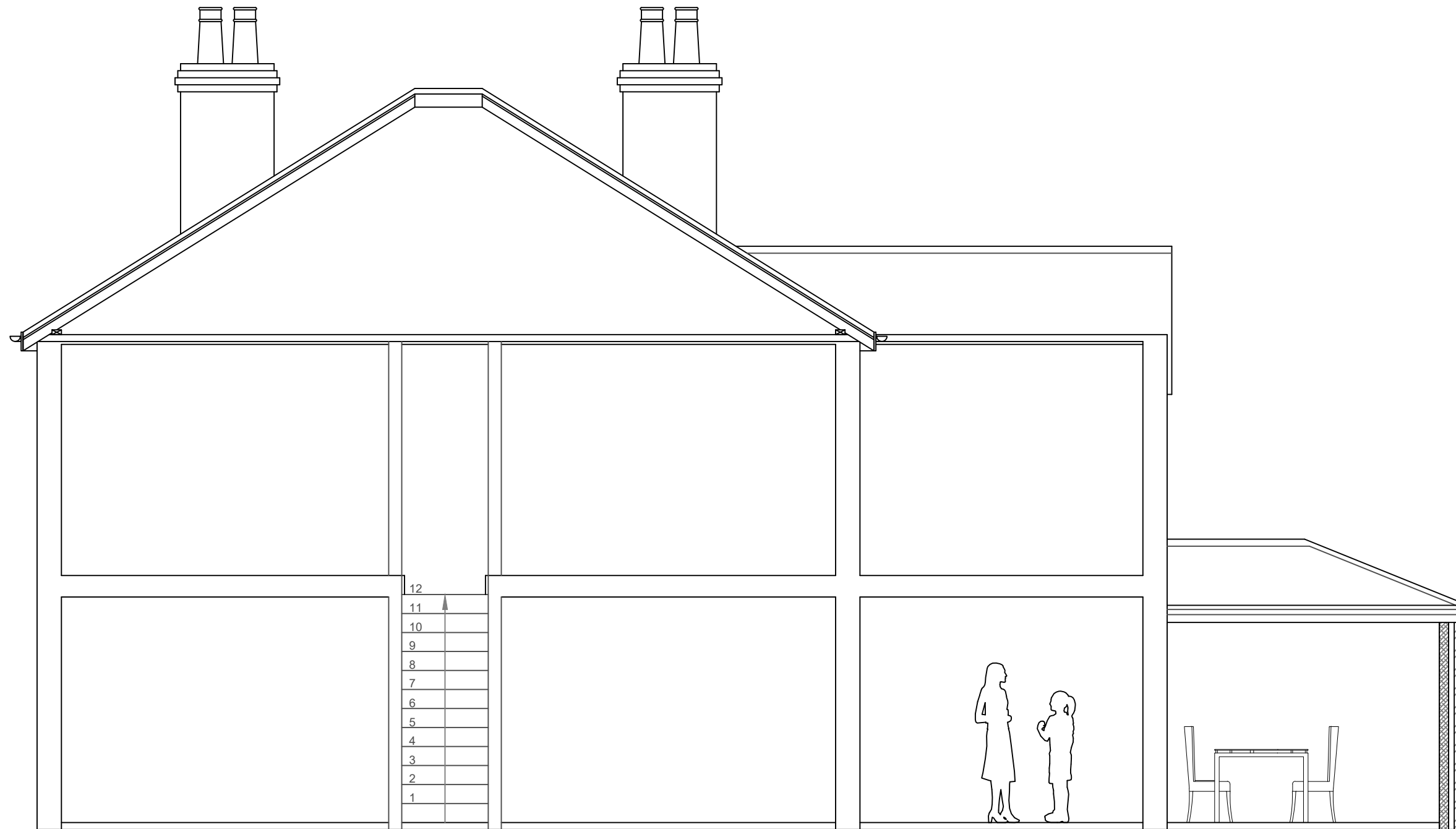
PROPOSED CROSS SECTION: AA SCALE 1:50
