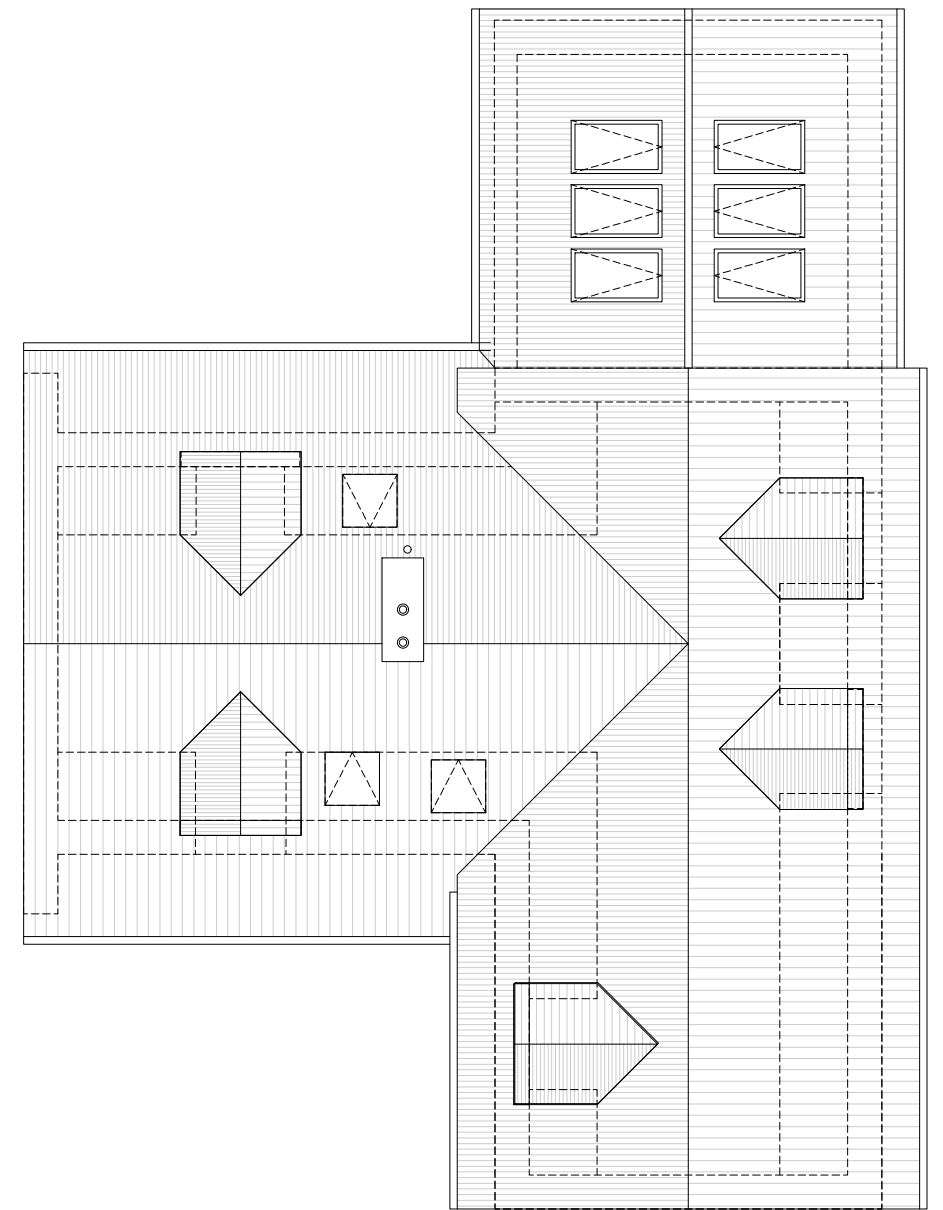
Roof Plan
