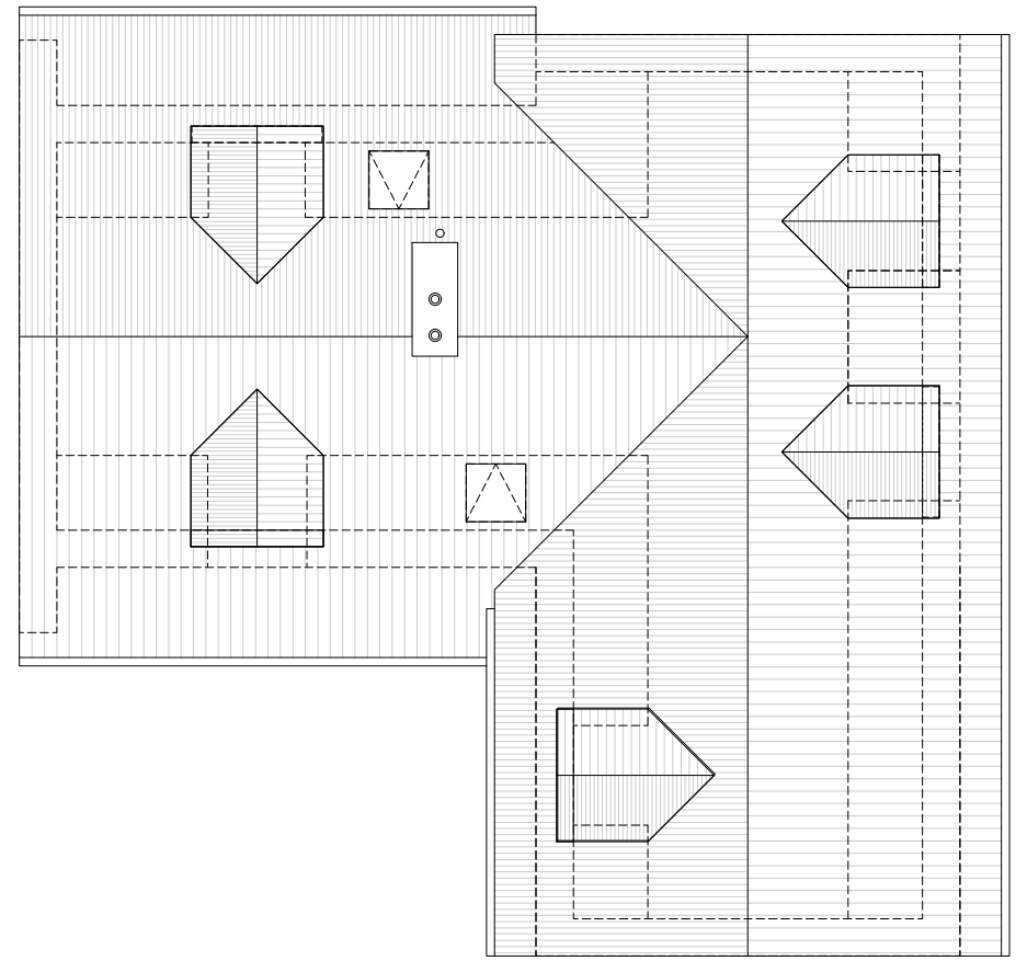
Roof Plan
