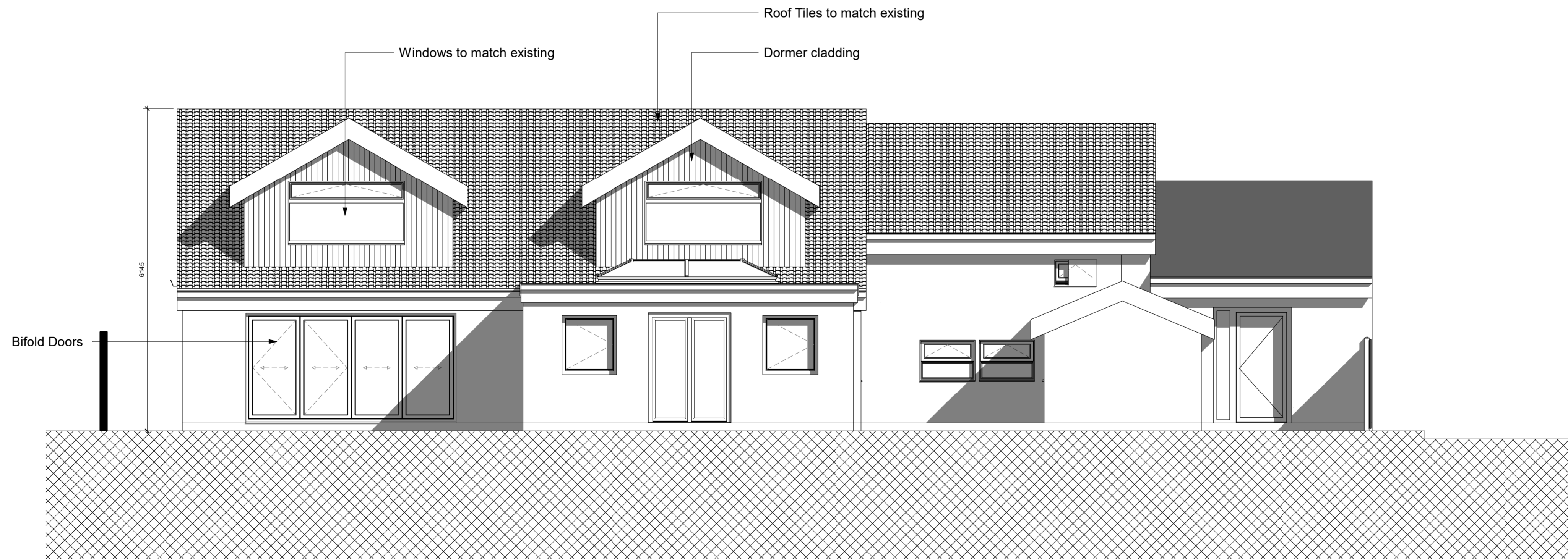
Proposed Rear Elevation 1 : 50
