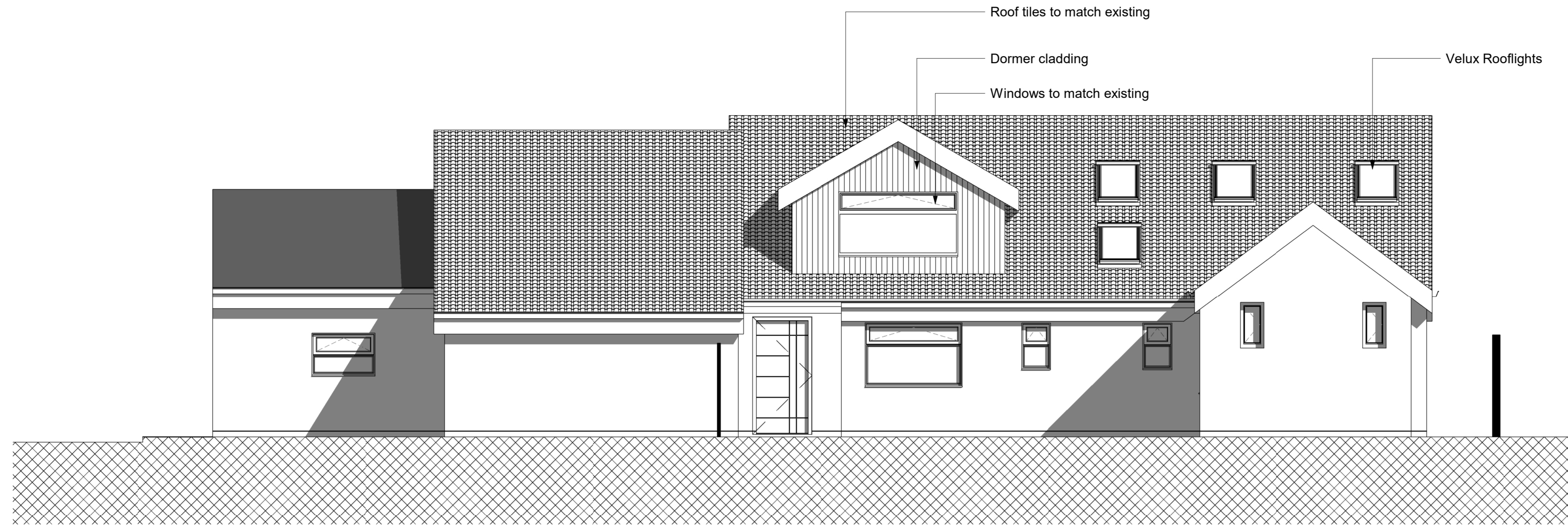
Proposed Front Elevation 1 : 50
