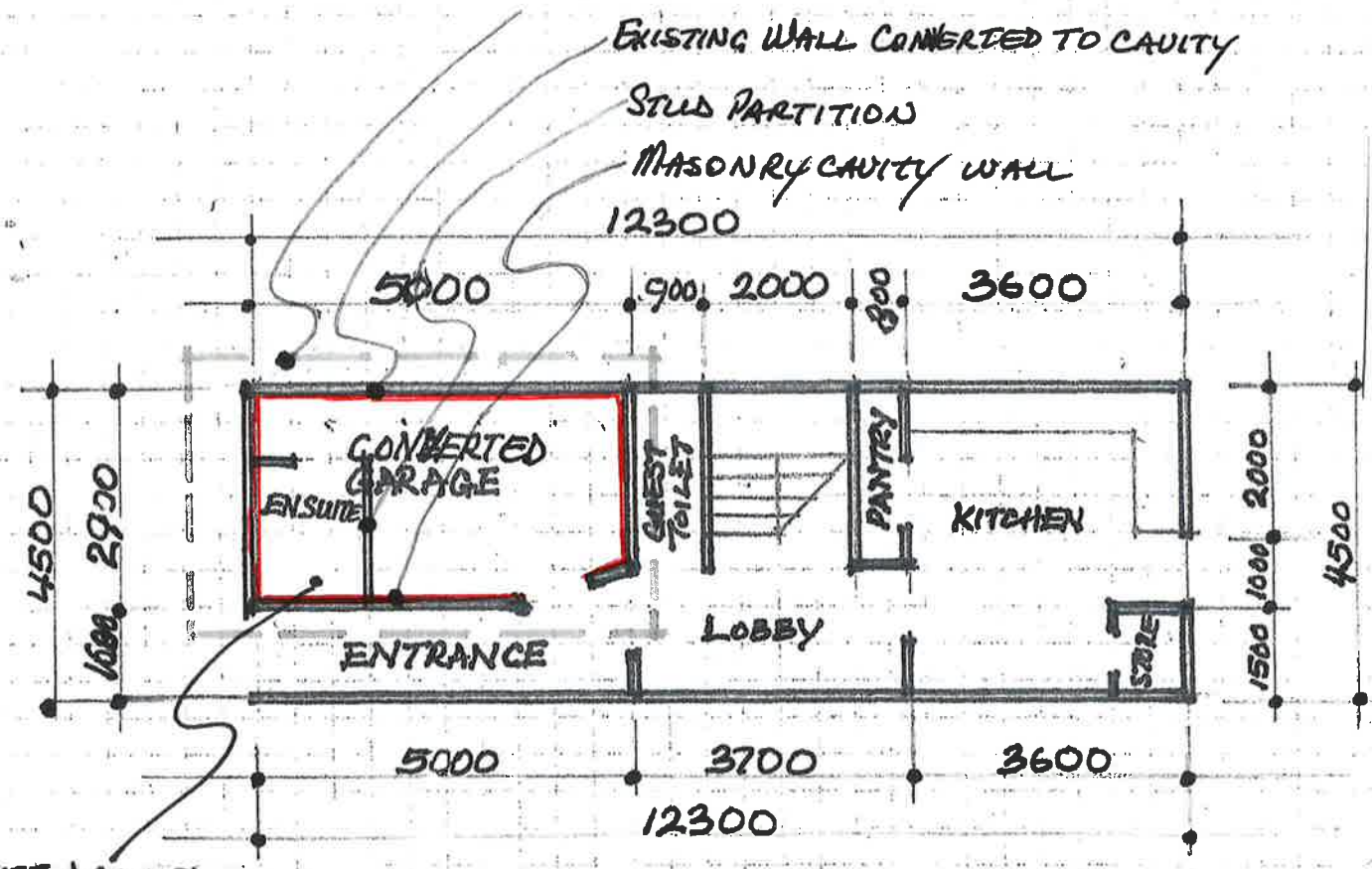
PROPOSED GRD FLR PLAN
