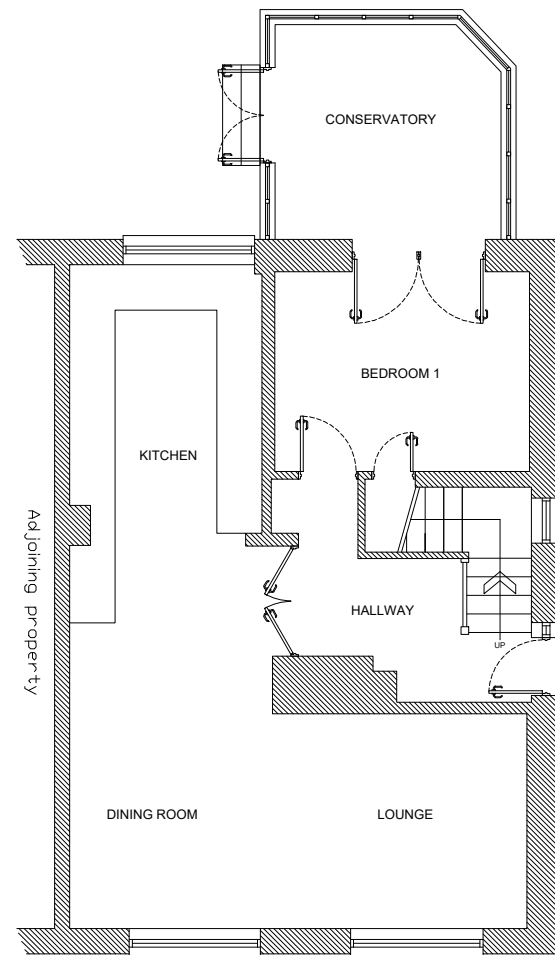
EXISTING GROUND FLOOR LAYOUT SCALE @ 1:100
