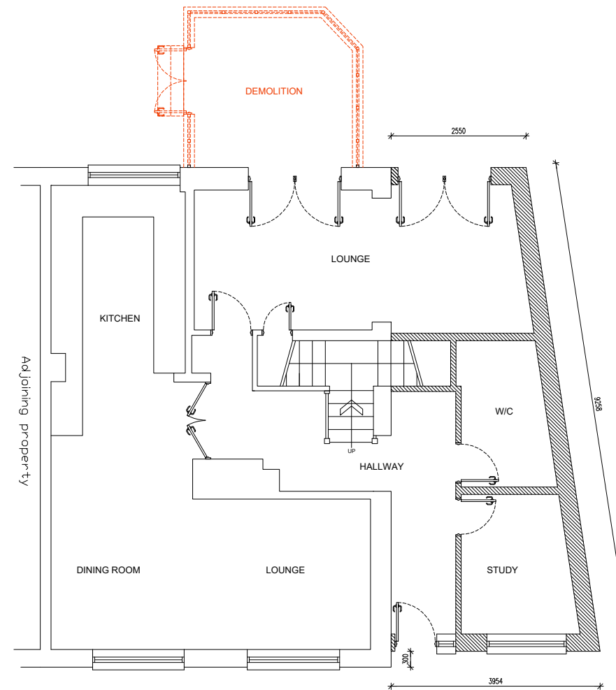
PROPOSED GROUND FLOOR LAYOUT SCALE @ 1:100
