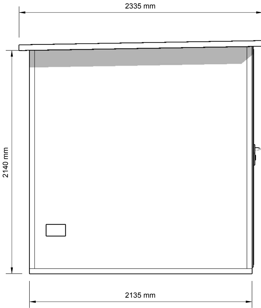
LEFTHAND ELEVATION
