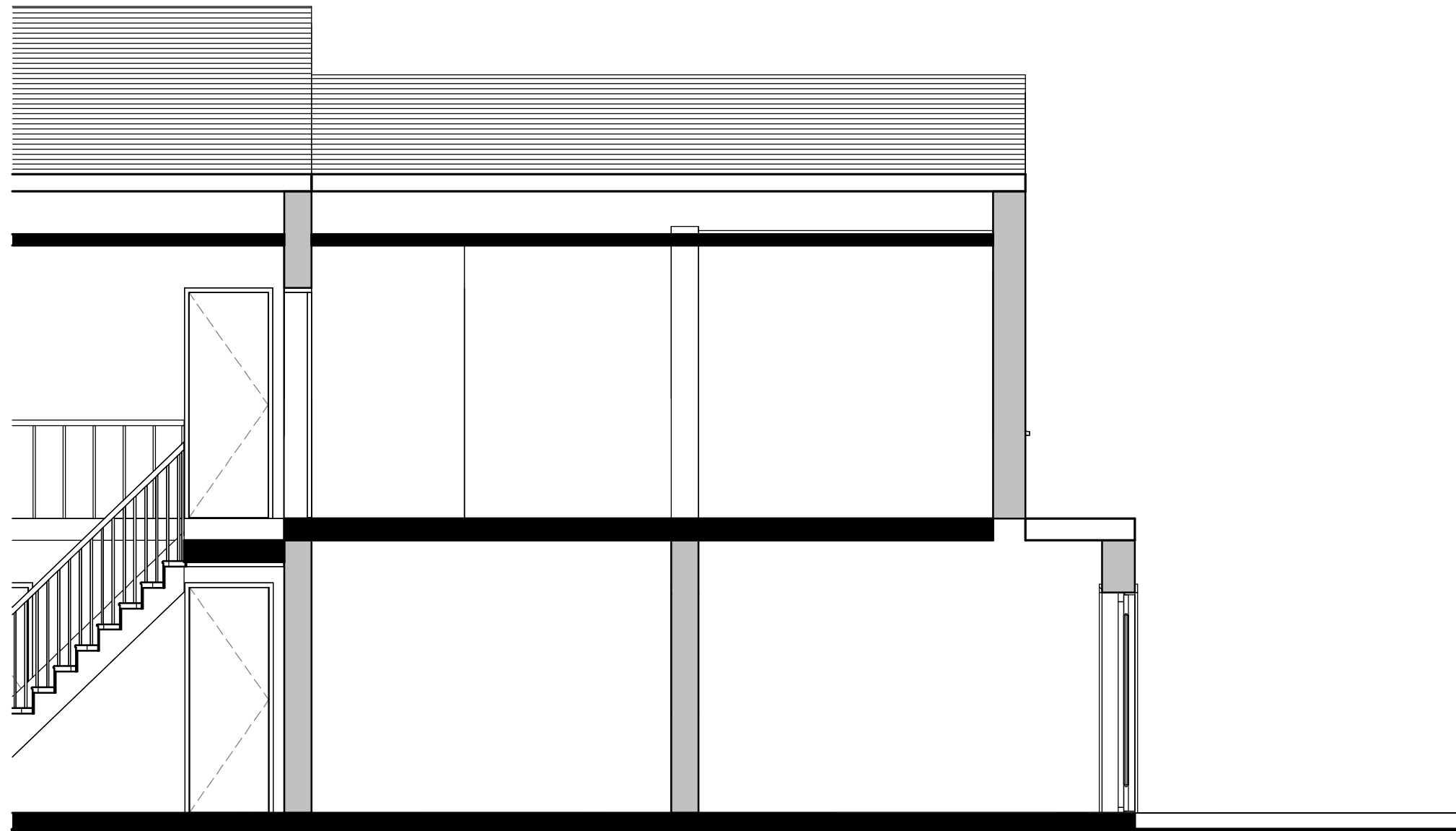
Proposed Section 1 1 : 50
