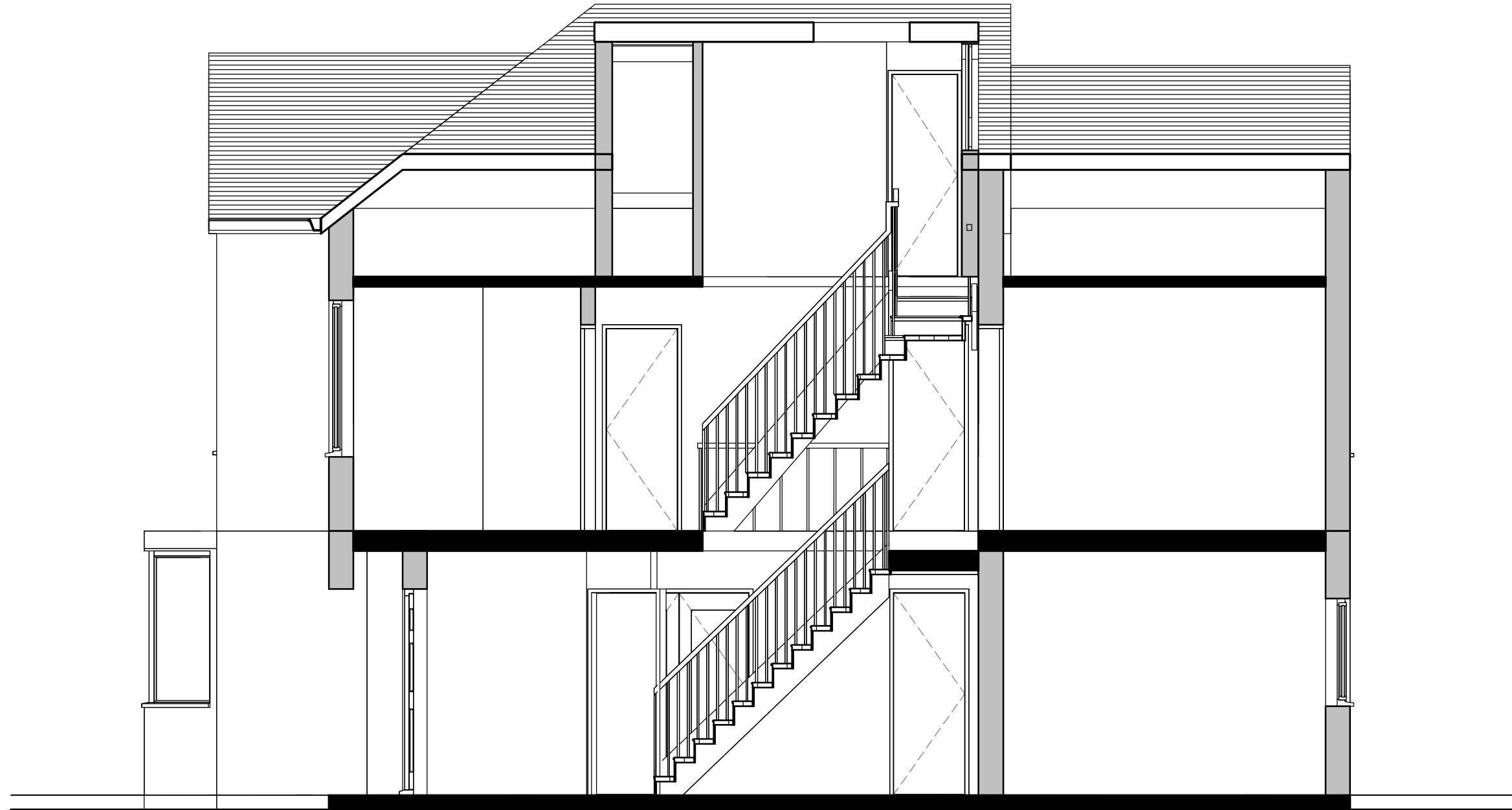
Proposed Section 1 1 : 50
