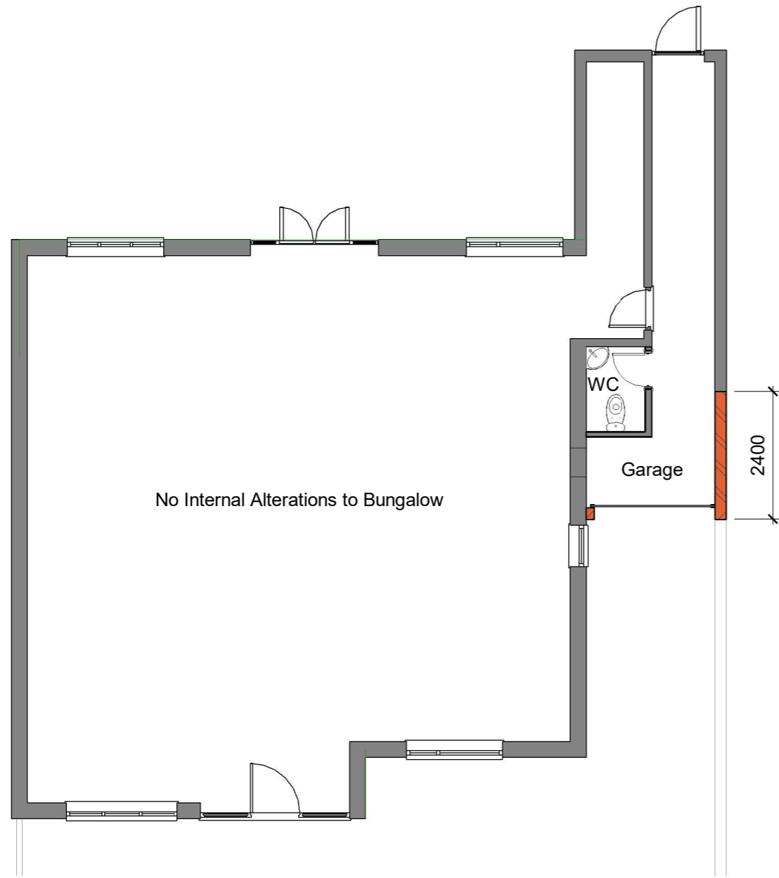
1 Ground Floor Layout 1 : 100
