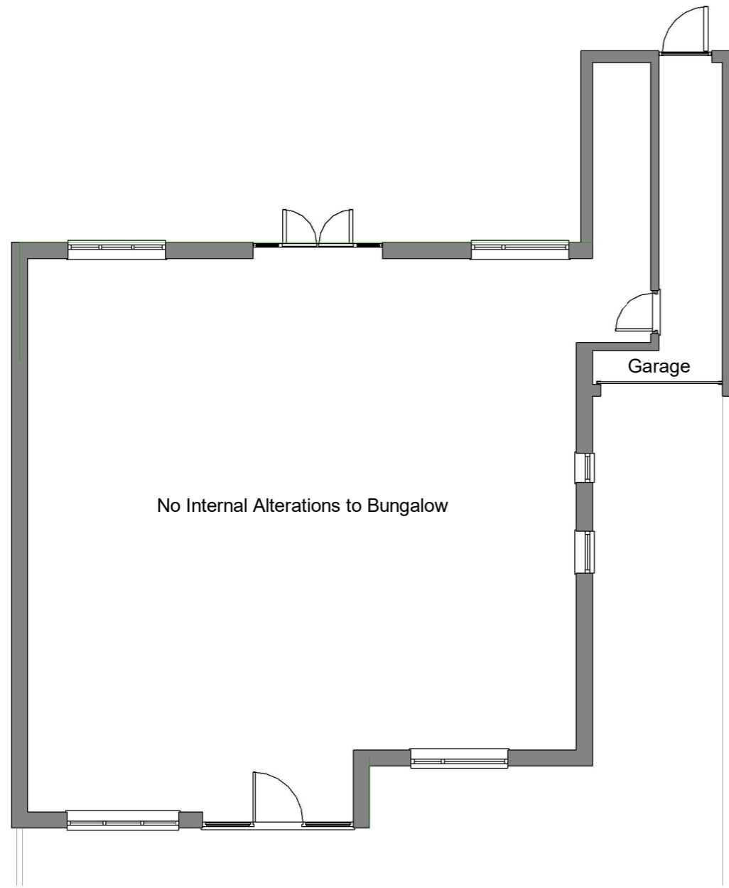
1 Ground Floor Layout 1 : 100
