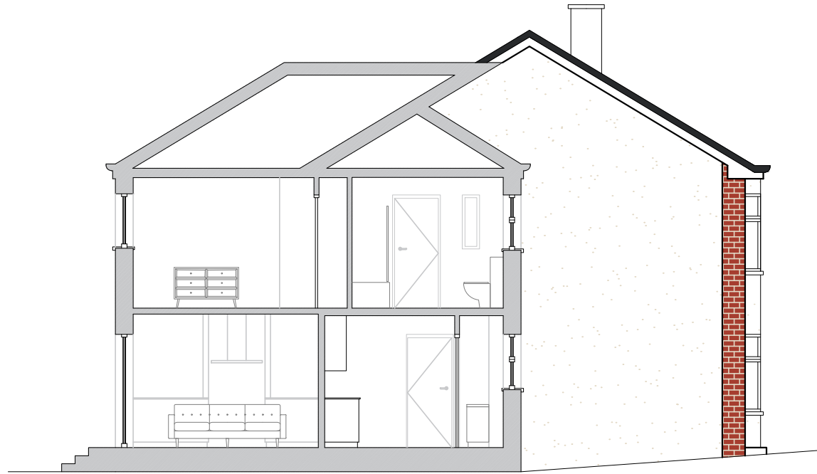
Existing Section C-C
