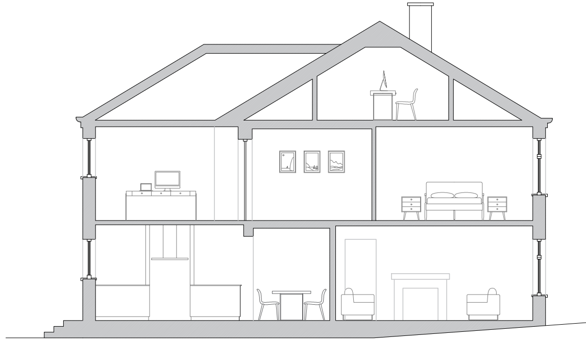
Existing Section D-D
