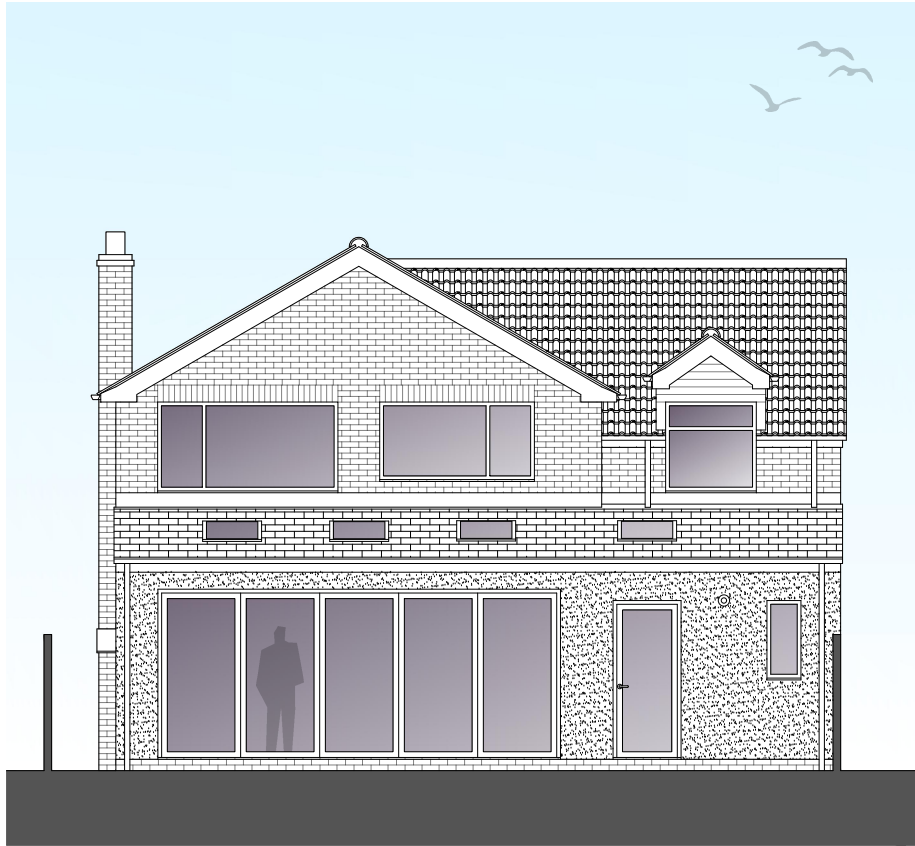
PROPOSED SOUTH EAST (REAR) ELEVATION
