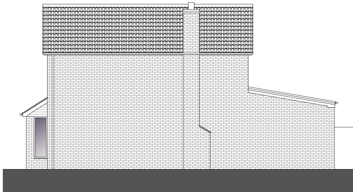
EXISTING SOUTH WEST (SIDE) ELEVATION
