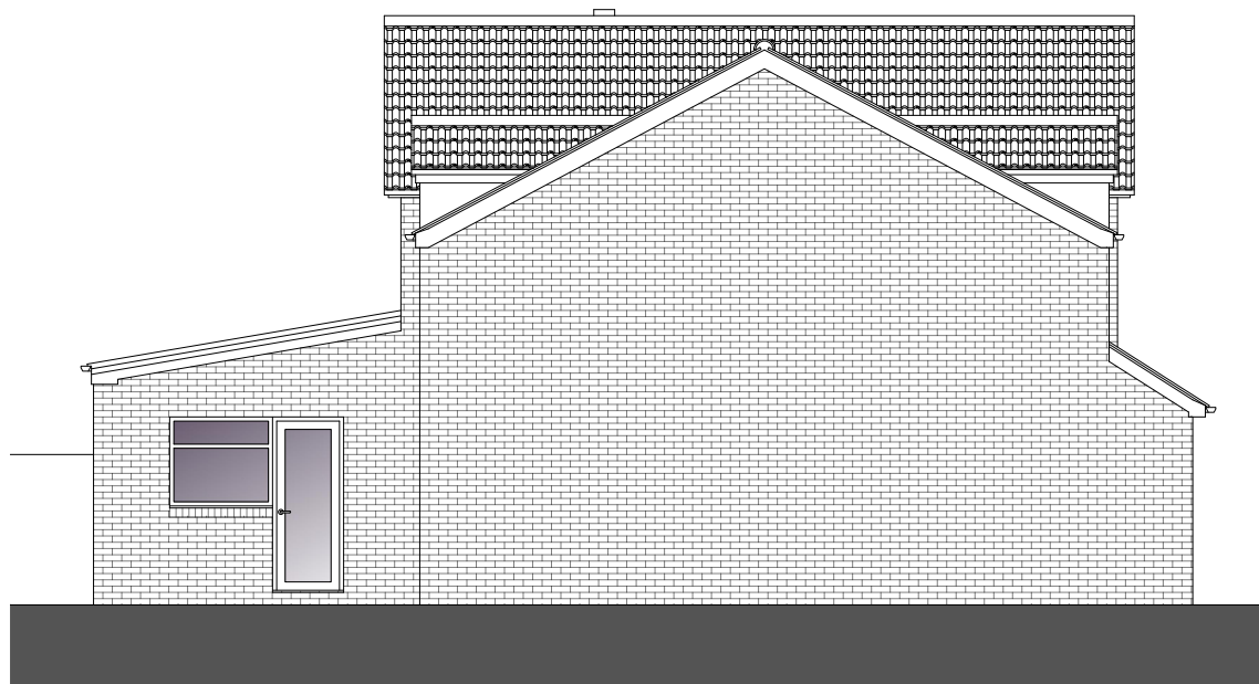
EXISTING NORTH EAST (SIDE) ELEVATION
